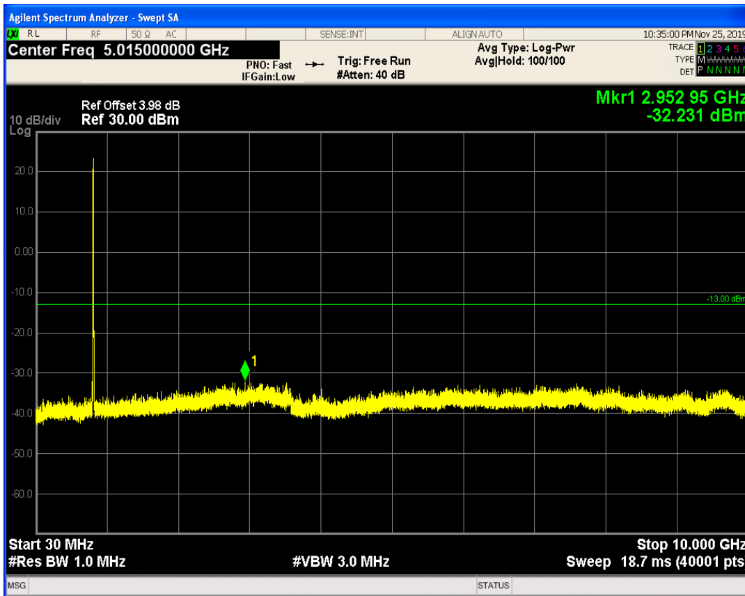
LTE Band19 QPSK BW=5MHz Channel=24025 RB Size=25 Position=#0
