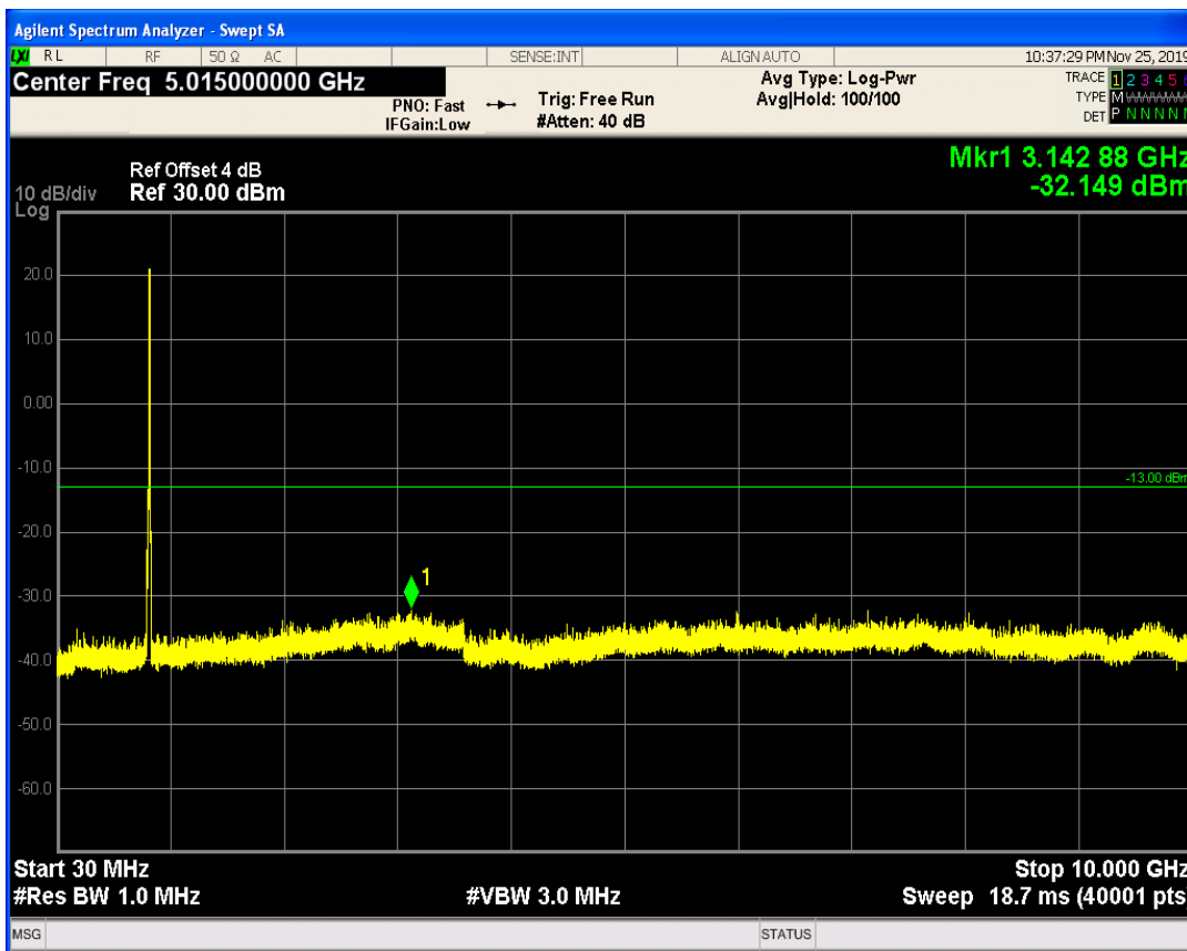
LTE Band19 QAM16 BW=10MHz Channel=24100 RB Size=50 Position=#0
