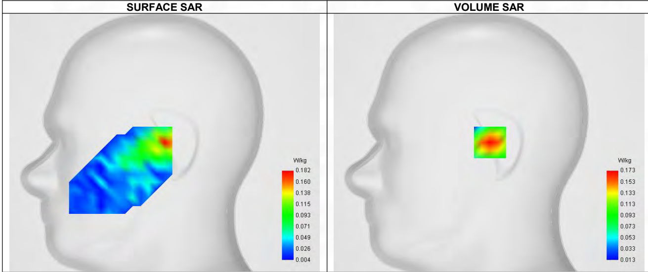
Maximum location: X=1.00, Y=0.00 ; SAR Peak: 0.29 W/kg
