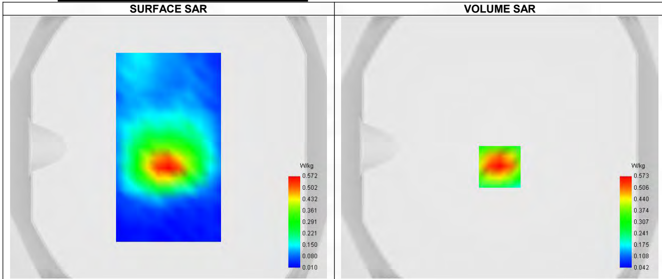
Maximum location: X=0.00, Y=-15.00 ; SAR Peak: 0.82 W/kg
