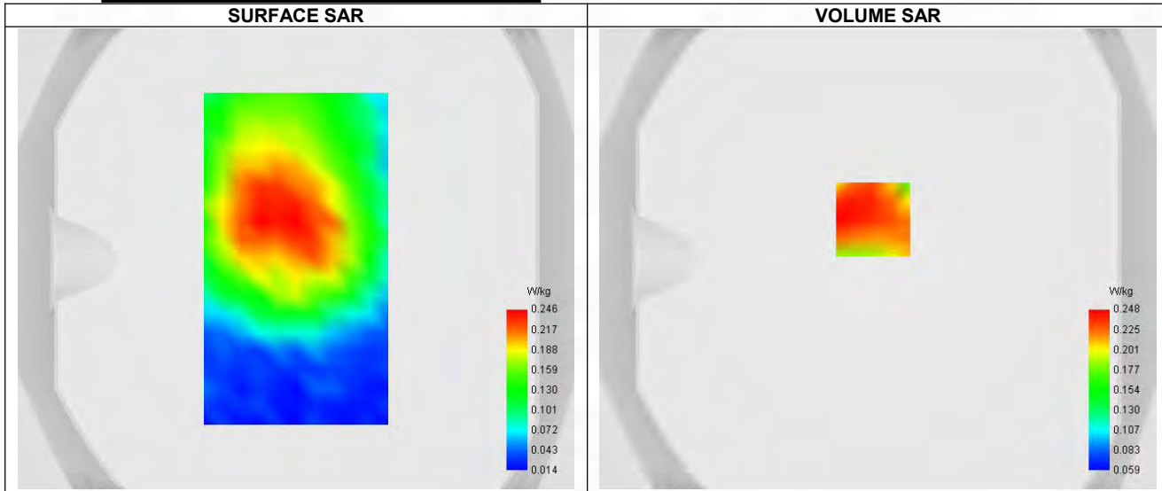
Maximum location: X=-2.00, Y=17.00 ; SAR Peak: 0.31 W/kg
