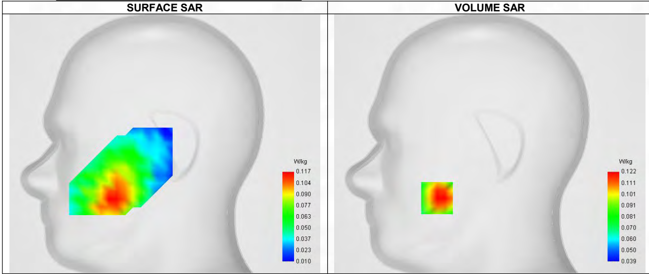
Maximum location: X=-53.00, Y=-55.00 ; SAR Peak: 0.17 W/kg
