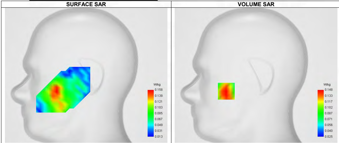
Maximum location: X=-57.00, Y=-31.00 ; SAR Peak: 0.20 W/kg
