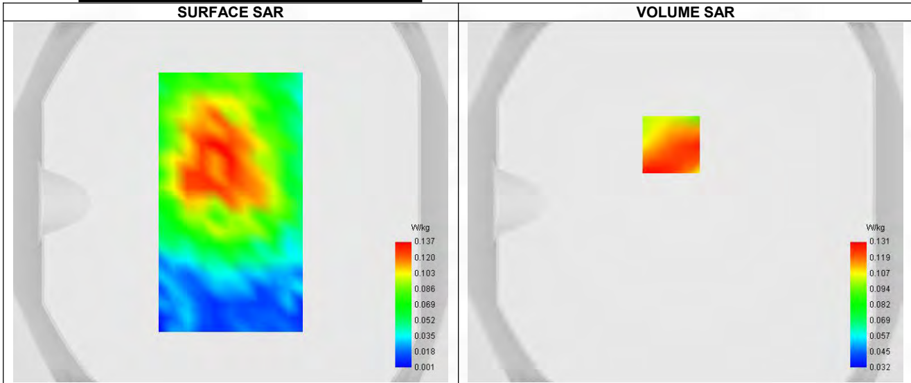
Maximum location: X=-8.00, Y=32.00 ; SAR Peak: 0.17 W/kg
