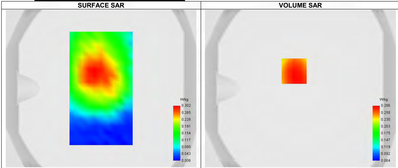
Maximum location: X=-8.00, Y=22.00 ; SAR Peak: 0.40 W/kg
