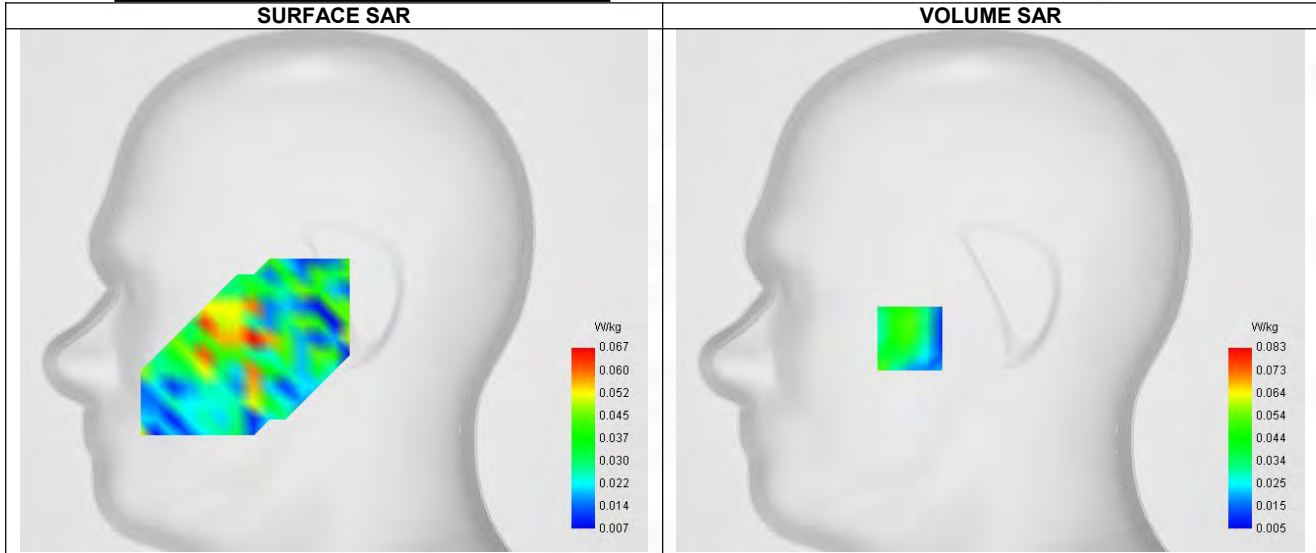
Maximum location: X=-40.00, Y=-24.00 ; SAR Peak: 0.11 W/kg
