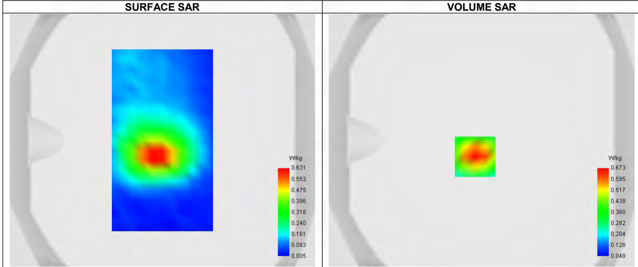
Maximum location: X=-5.00, Y=-13.00 ; SAR Peak: 0.99 W/kg
