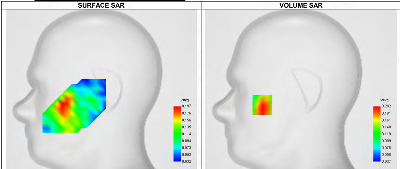
Maximum location: X=-63.00, Y=-26.00 ; SAR Peak: 0.31 W/kg
