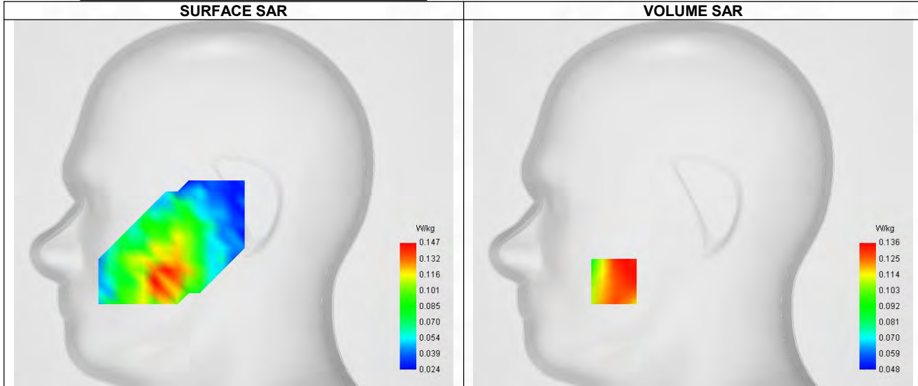
Maximum location: X=-56.00, Y=-56.00 ; SAR Peak: 0.19 W/kg
