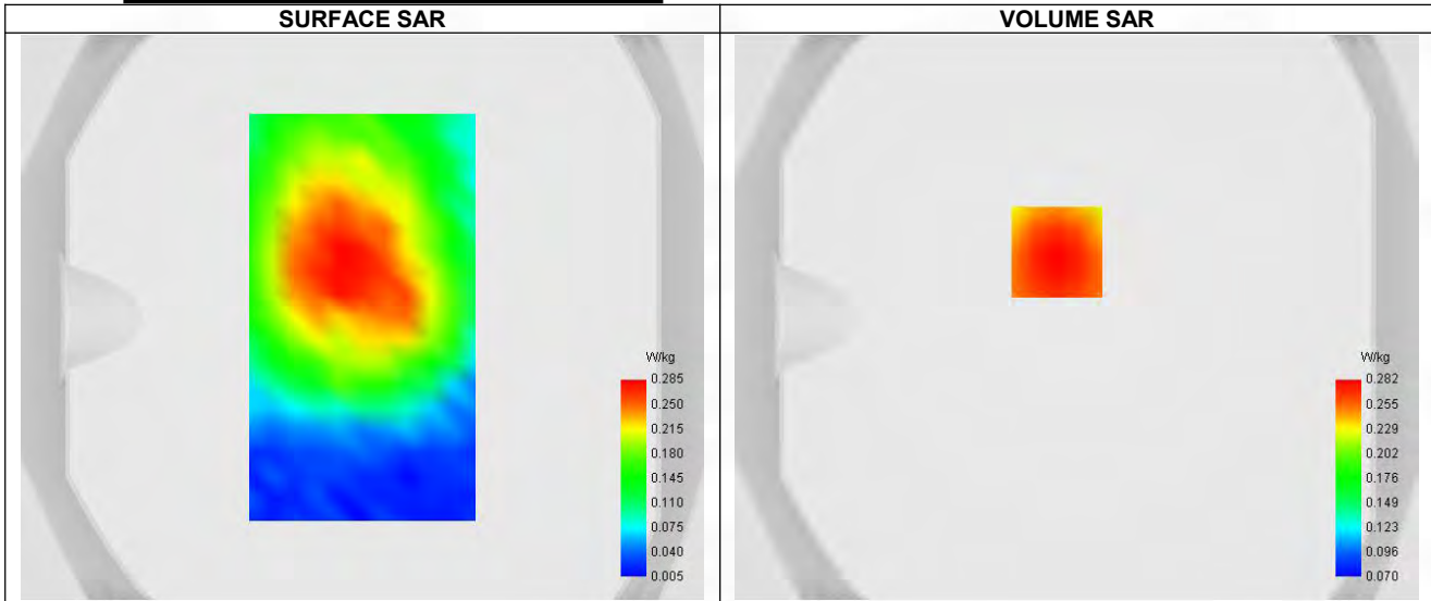
Maximum location: X=-7.00, Y=23.00 ; SAR Peak: 0.37 W/kg
