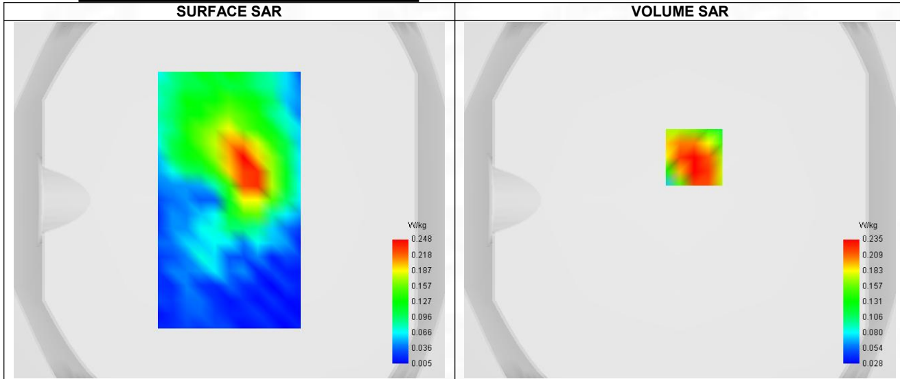
Maximum location: X=8.00, Y=24.00 ; SAR Peak: 0.32 W/kg
