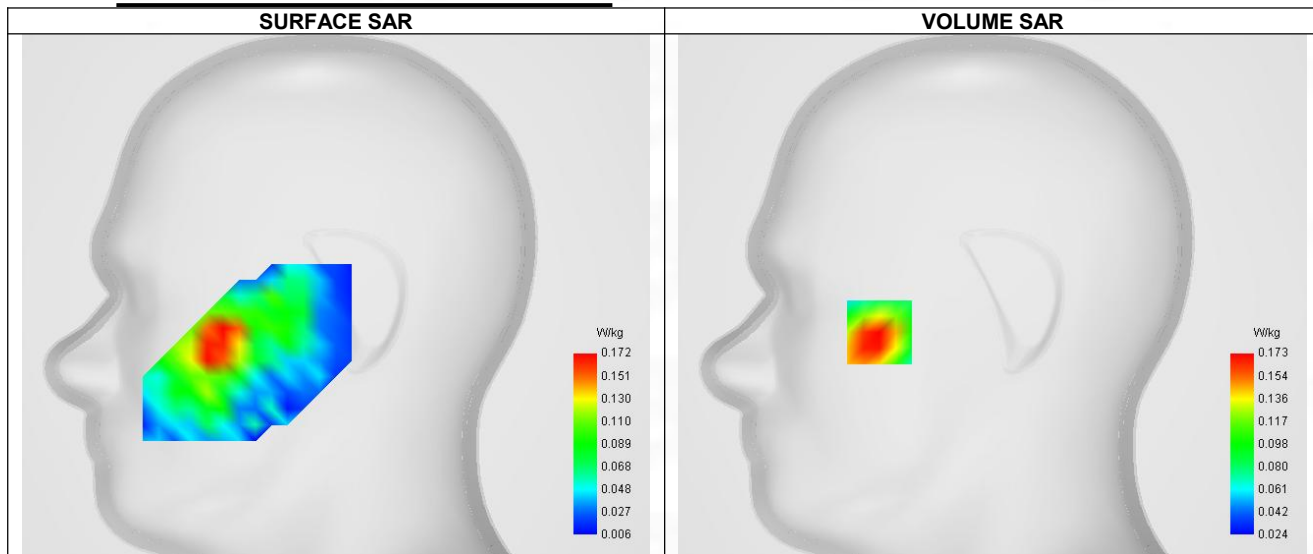
Maximum location: X=-56.00, Y=-18.00 ; SAR Peak: 0.24 W/kg
