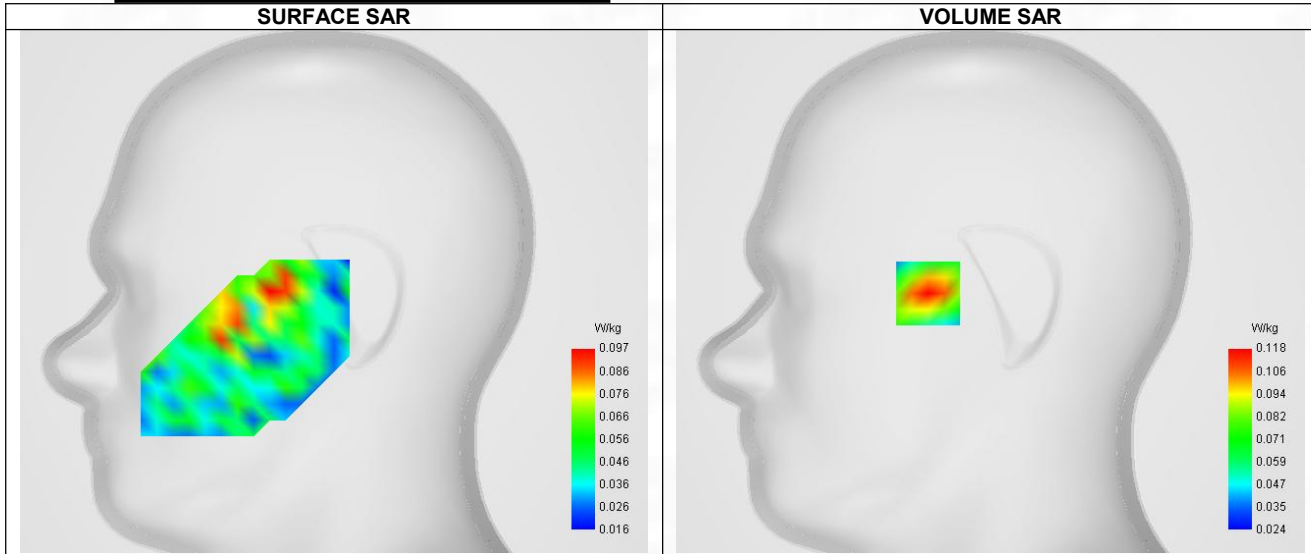
Maximum location: X=-31.00, Y=-1.00 ; SAR Peak: 0.16 W/kg
