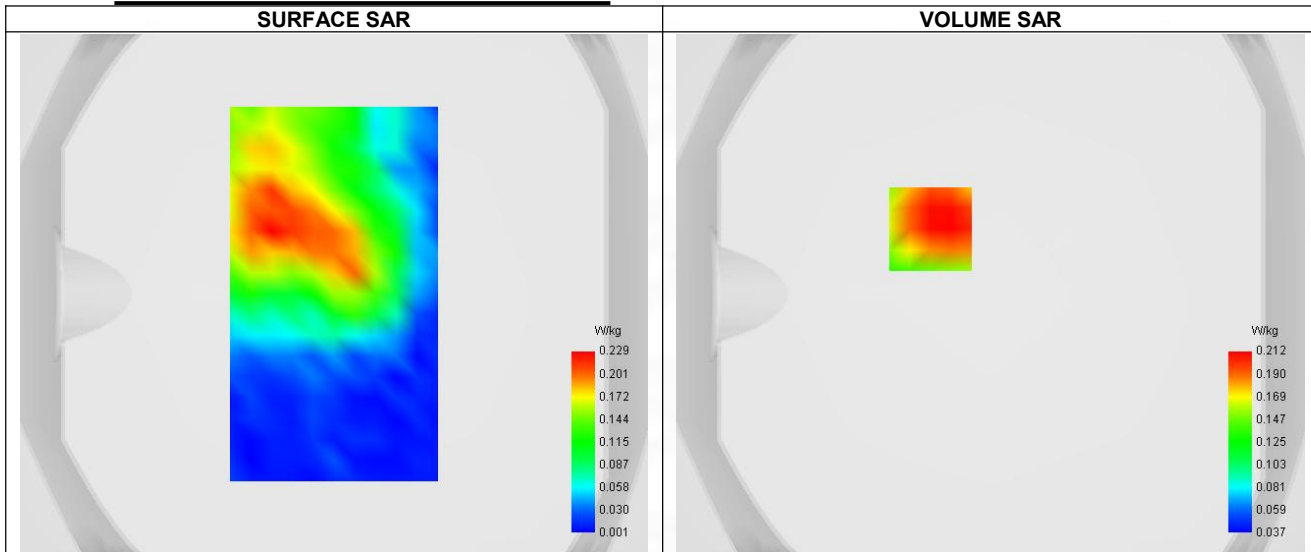
Maximum location: X=-23.00, Y=25.00 ; SAR Peak: 0.30 W/kg
