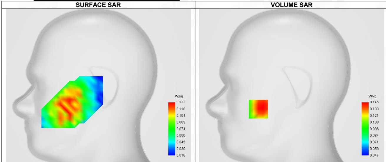
Maximum location: X=-56.00, Y=-40.00 ; SAR Peak: 0.19 W/kg
