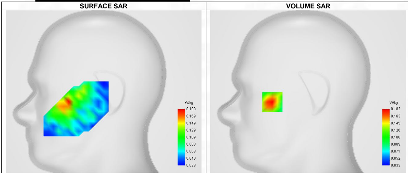
Maximum location: X=-57.00, Y=-17.00 ; SAR Peak: 0.27 W/kg
