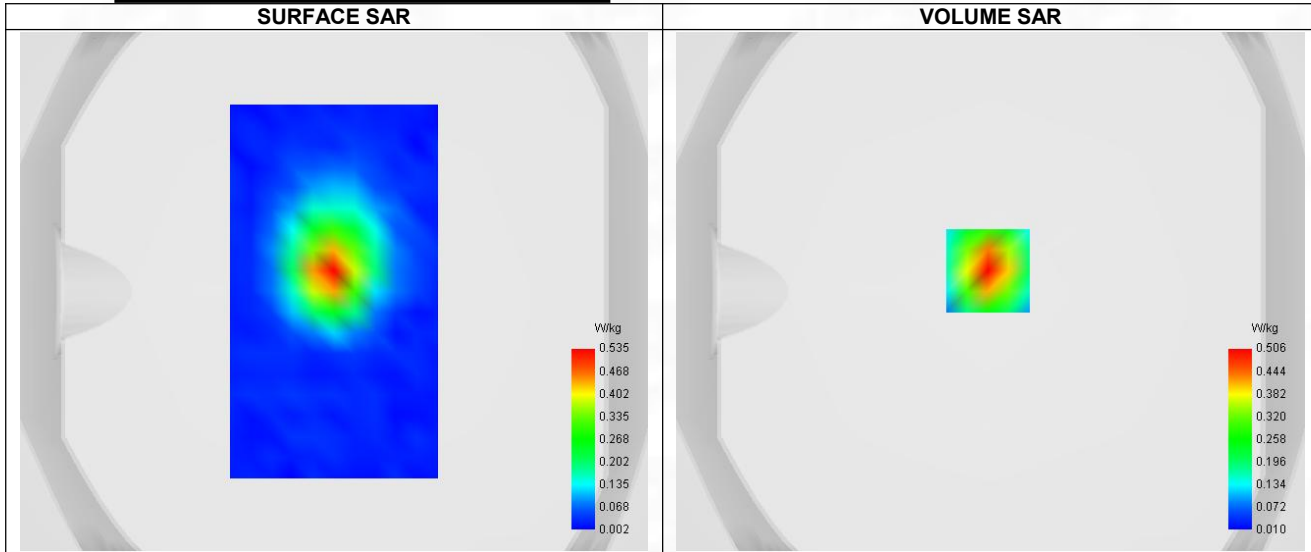
Maximum location: X=-1.00, Y=8.00 ; SAR Peak: 0.77 W/kg
