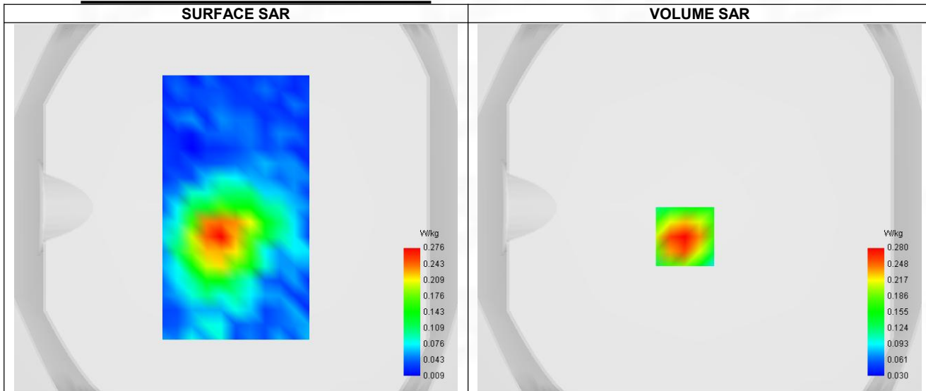
Maximum location: X=-8.00, Y=-16.00 ; SAR Peak: 0.44 W/kg
