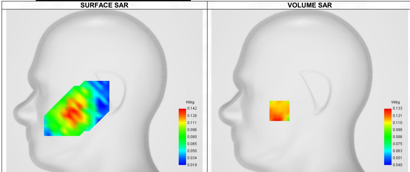
Maximum location: X=-48.00, Y=-32.00 ; SAR Peak: 0.17 W/kg
