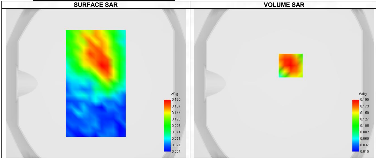
Maximum location: X=9.00, Y=24.00 ; SAR Peak: 0.26 W/kg
