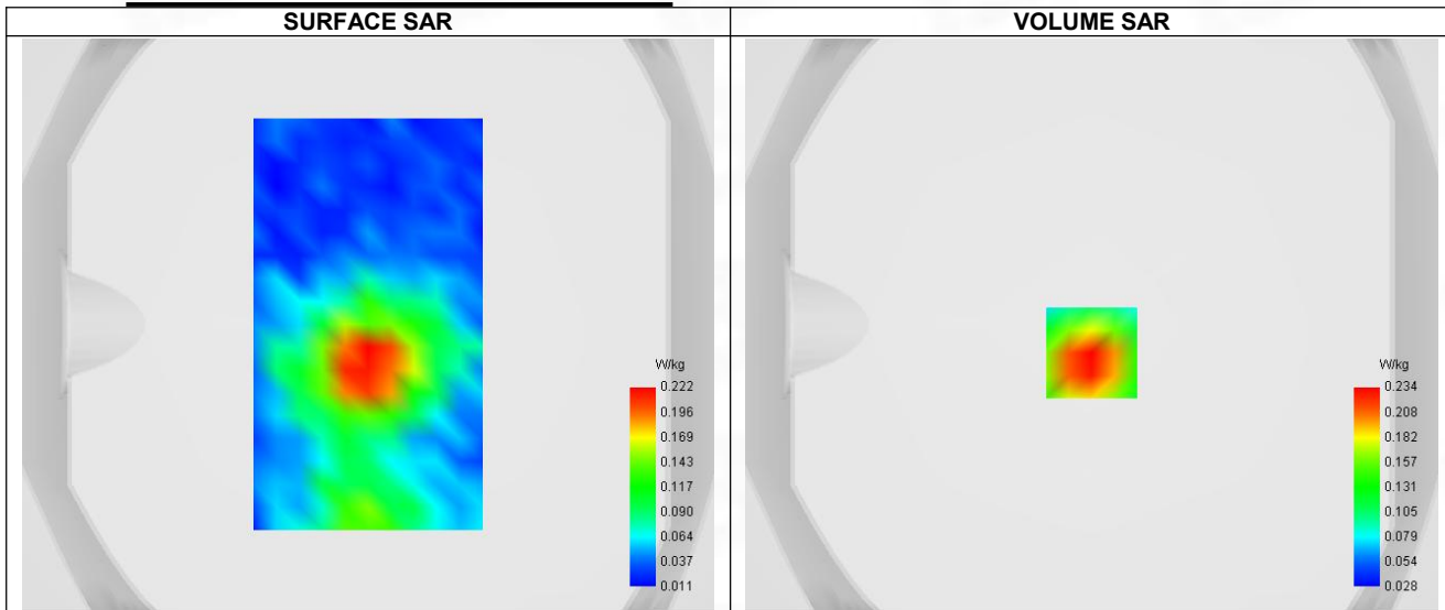
Maximum location: X=0.00, Y=-10.00 ; SAR Peak: 0.36 W/kg
