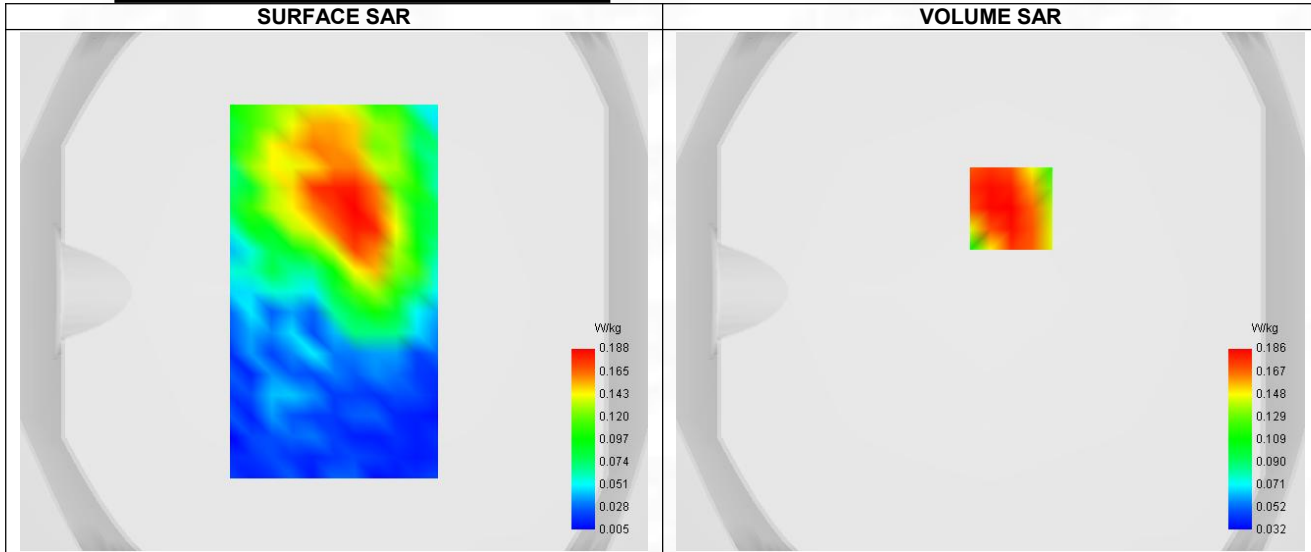
Maximum location: X=8.00, Y=32.00 ; SAR Peak: 0.26 W/kg
