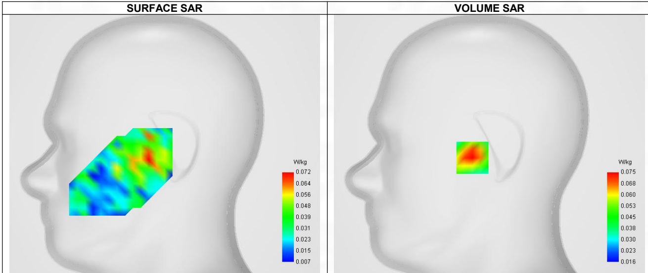
Maximum location: X=-17.00, Y=-14.00 ; SAR Peak: 0.10 W/kg
