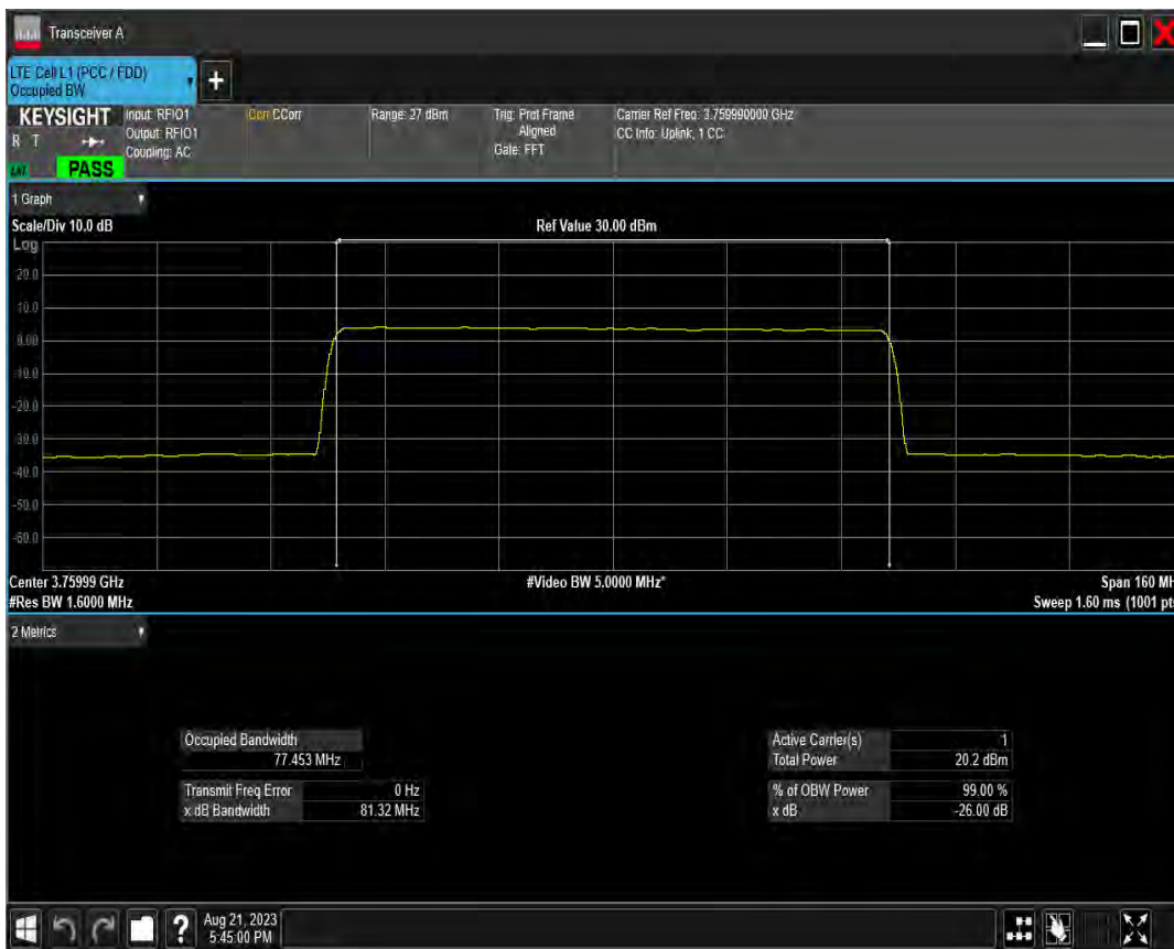
n78(3700-3800) SCS=30kHz DFT 256QAM BW=80MHz Channel=650000 RB=216@0
