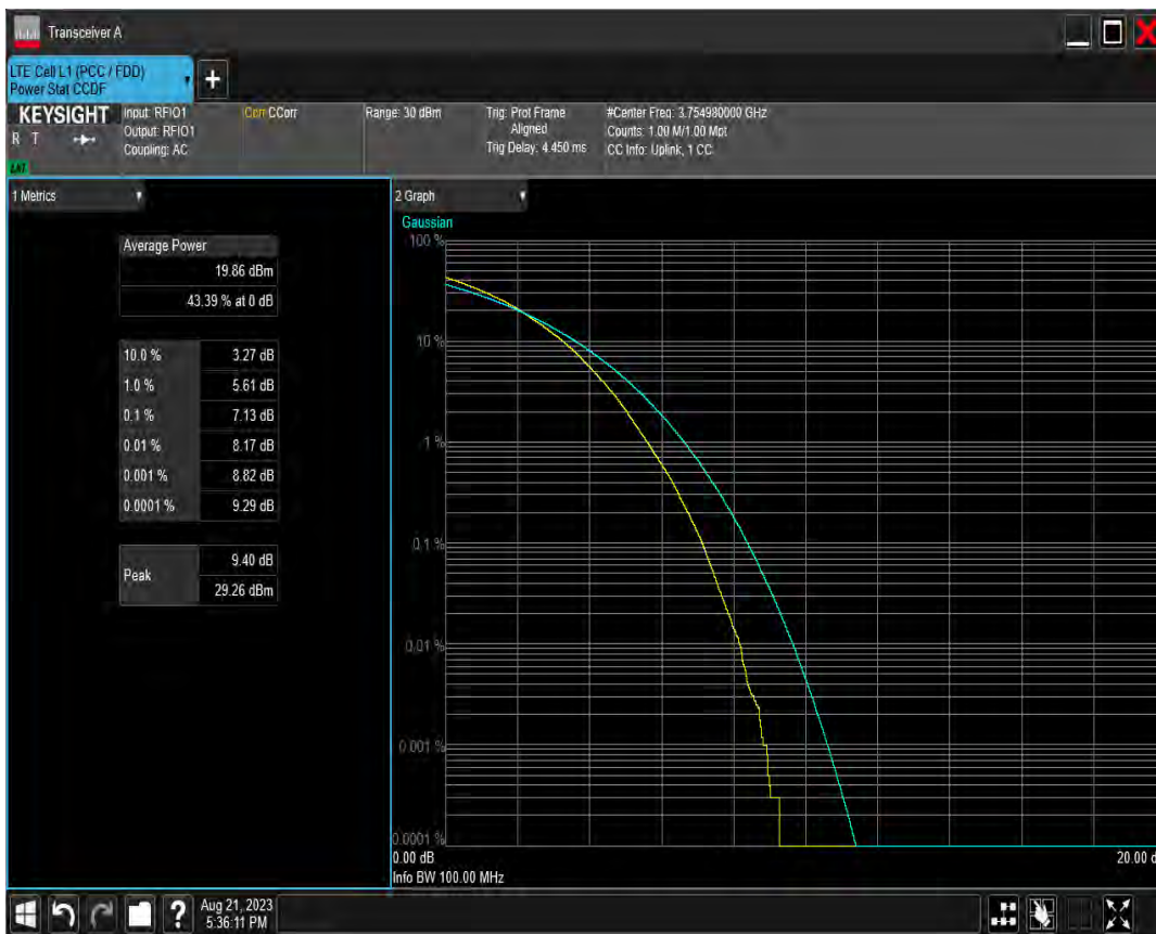
n78(3700-3800) SCS=30kHz DFT 64QAM BW=100MHz Channel=650000 RB=270@0
