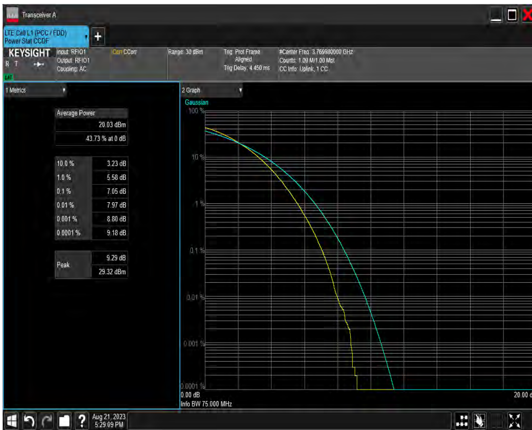
n78(3700-3800) SCS=30kHz DFT 256QAM BW=80MHz Channel=650666 RB=216@0
