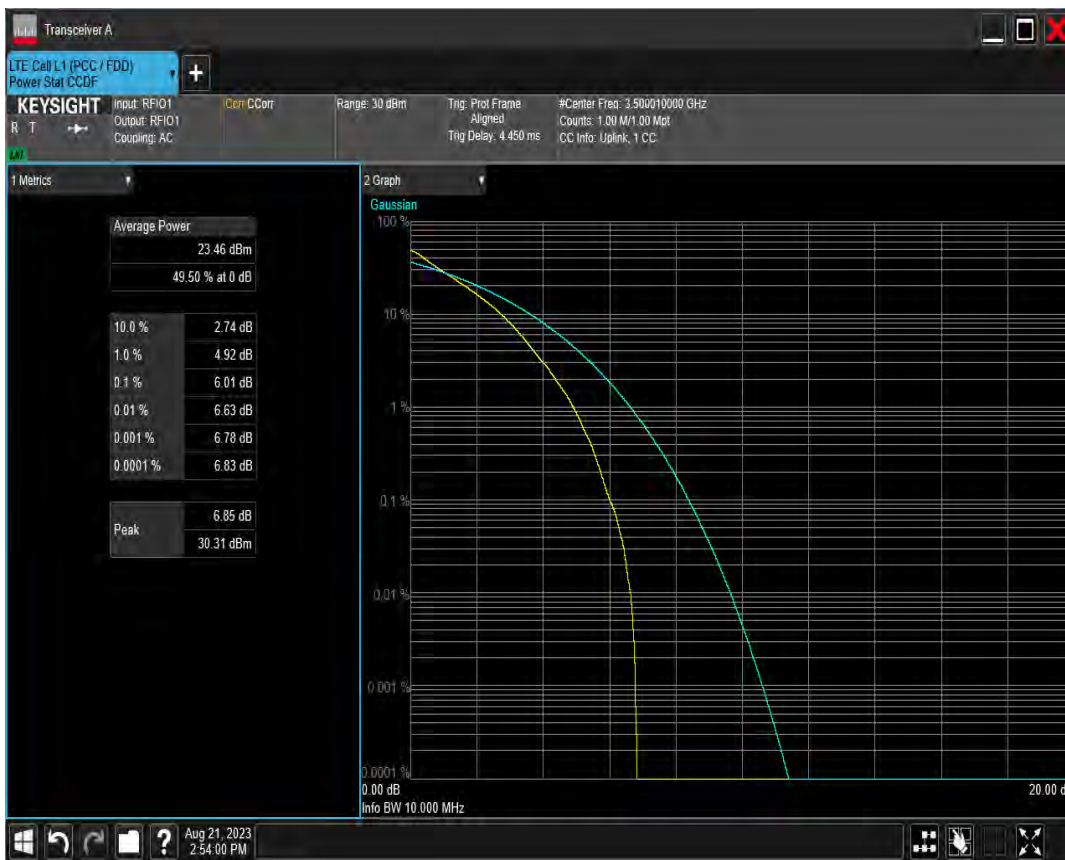
n78(3450-3550) SCS=30kHz DFT QPSK BW=10MHz Channel=633332 RB=24 @ 0
