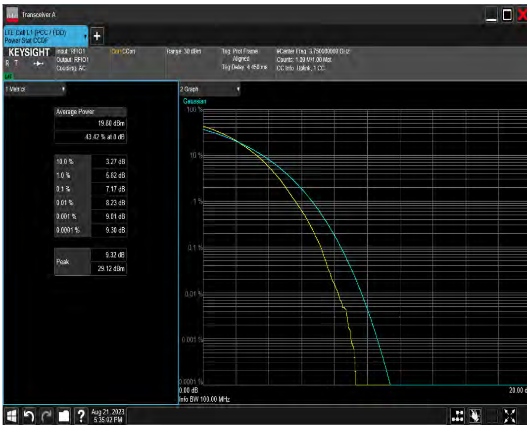
n78(3700-3800) SCS=30kHz DFT 256QAM BW=90MHz Channel=650332 RB=240@0
