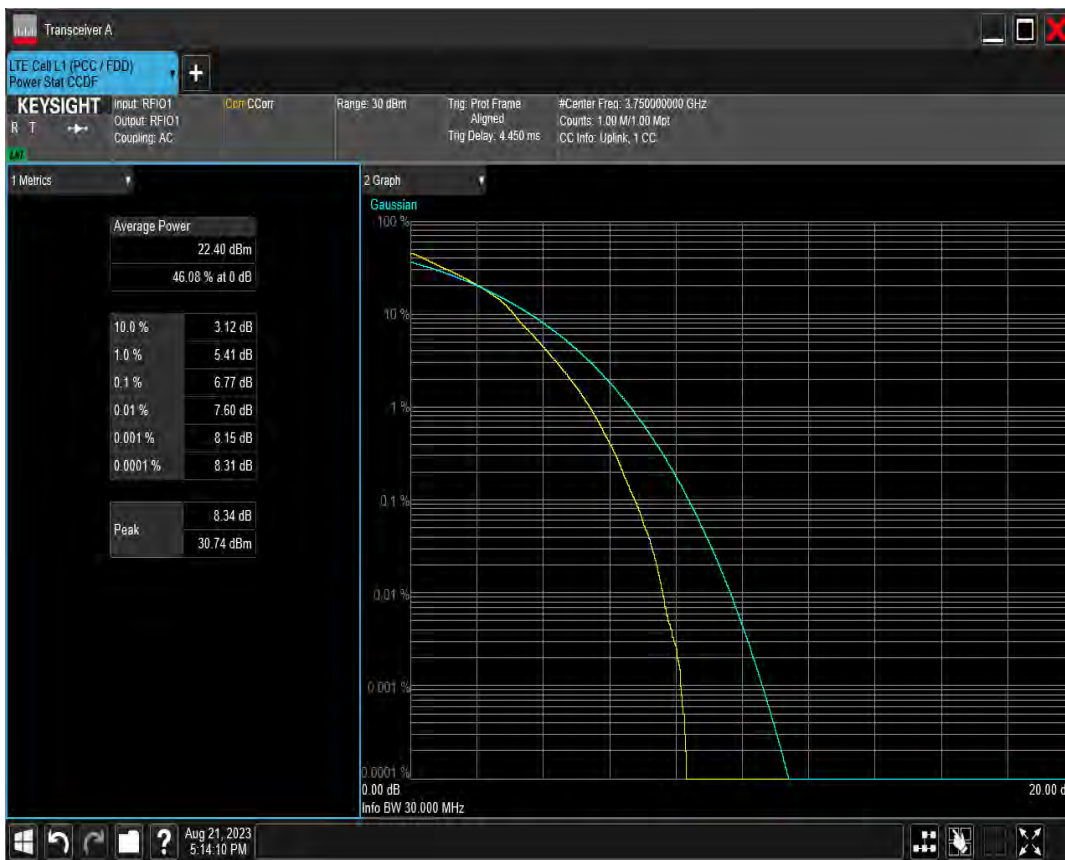
n78(3700-3800) SCS=30kHz DFT 16QAM BW=30MHz Channel=647668 RB=75@0
