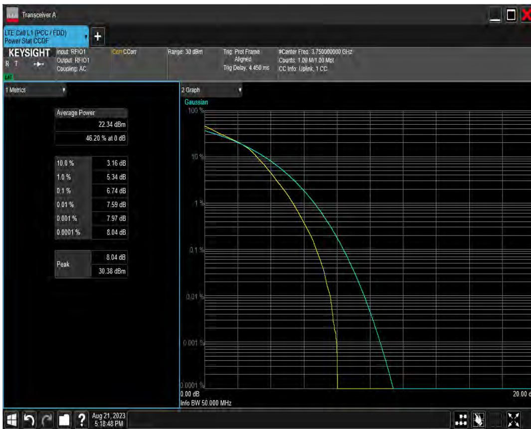
n78(3700-3800) SCS=30kHz DFT 16QAM BW=50MHz Channel=651666 RB=128@0
