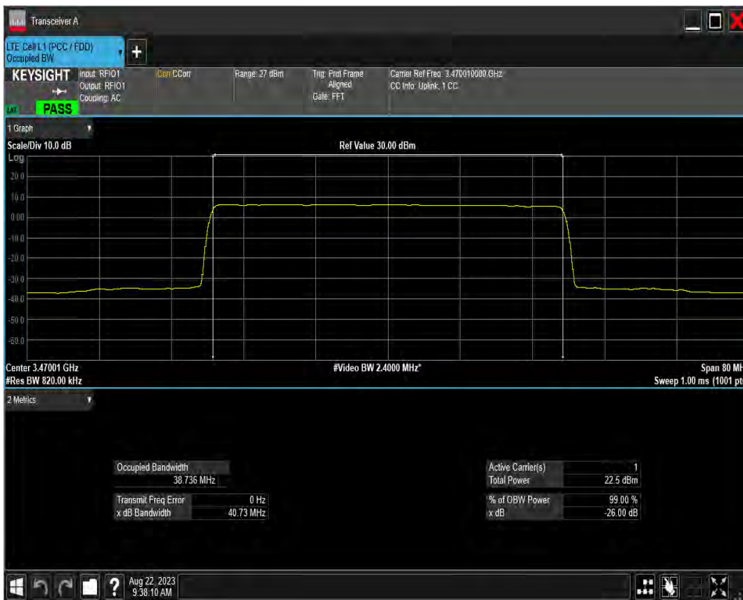
n78(3450-3550) SCS=15kHz DFT 64QAM BW=40MHz Channel=633334 RB=216@0
