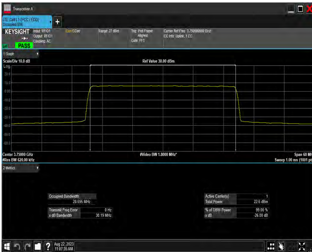
n78(3700-3800) SCS=15kHz DFT 16QAM BW=40MHz Channel=650000 RB=216@0
