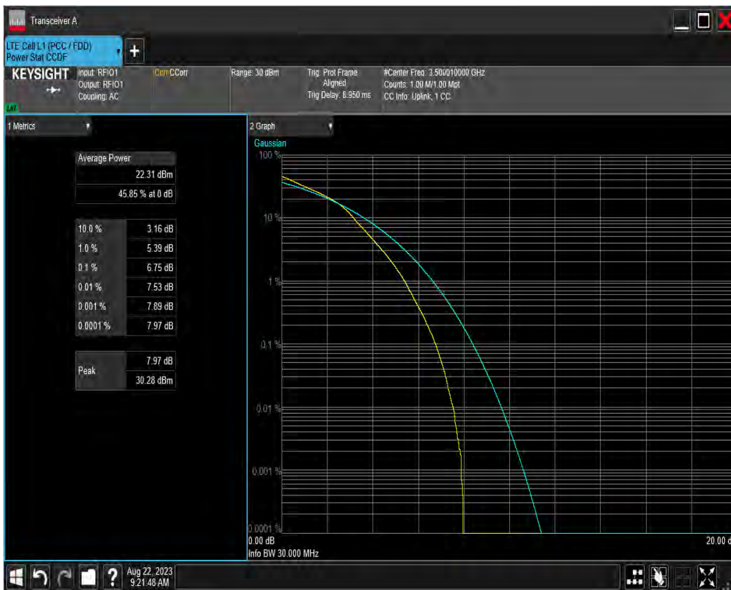
n78(3450-3550) SCS=15kHz DFT 16QAM BW=40MHz Channel=633334 RB=216@0
