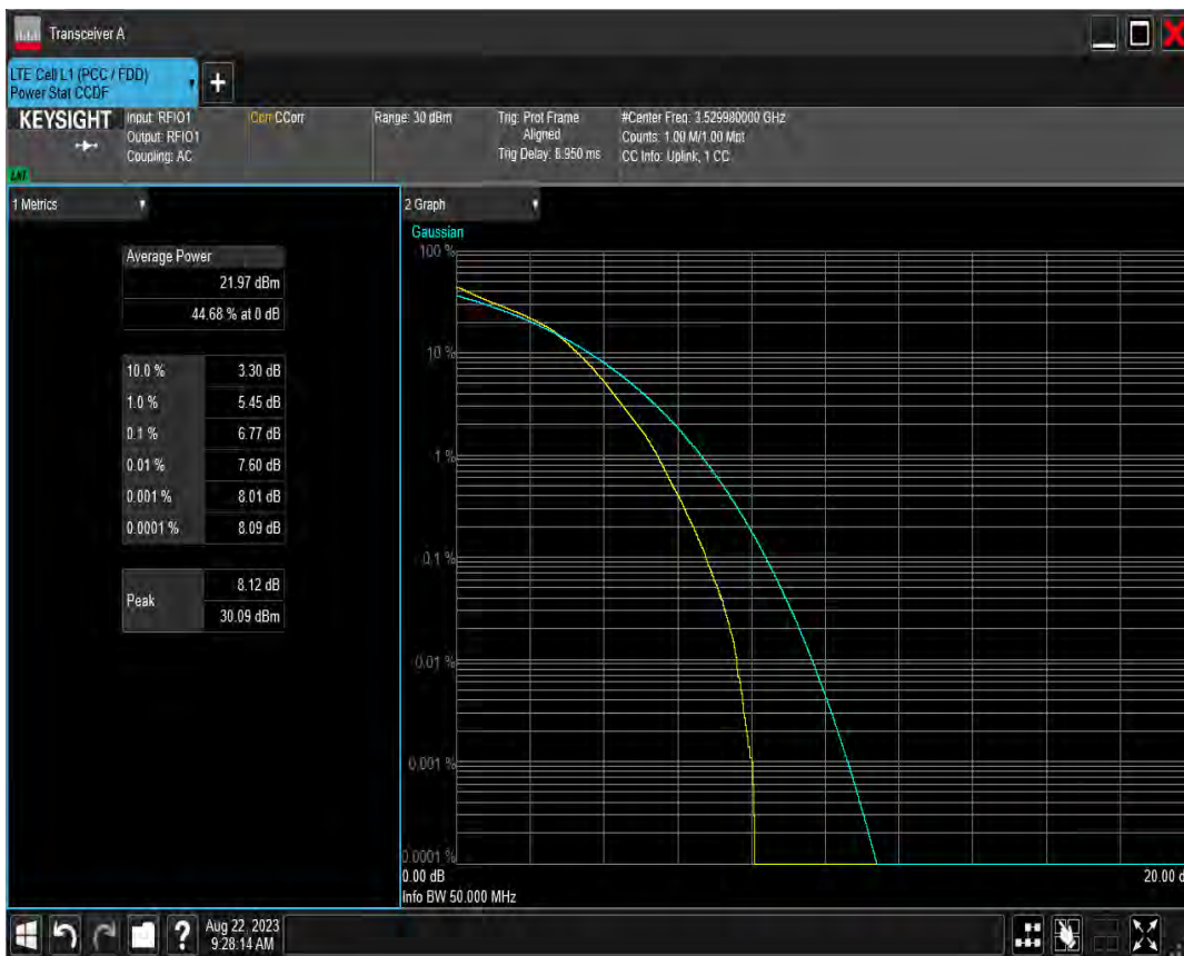
n78(3450-3550) SCS=15kHz DFT 16QAM BW=50MHz Channel=631668 RB=270@0
