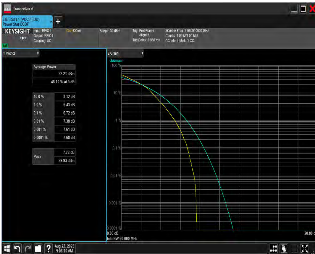
n78(3450-3550) SCS=15kHz DFT 16QAM BW=15MHz Channel=636166 RB=75@0
