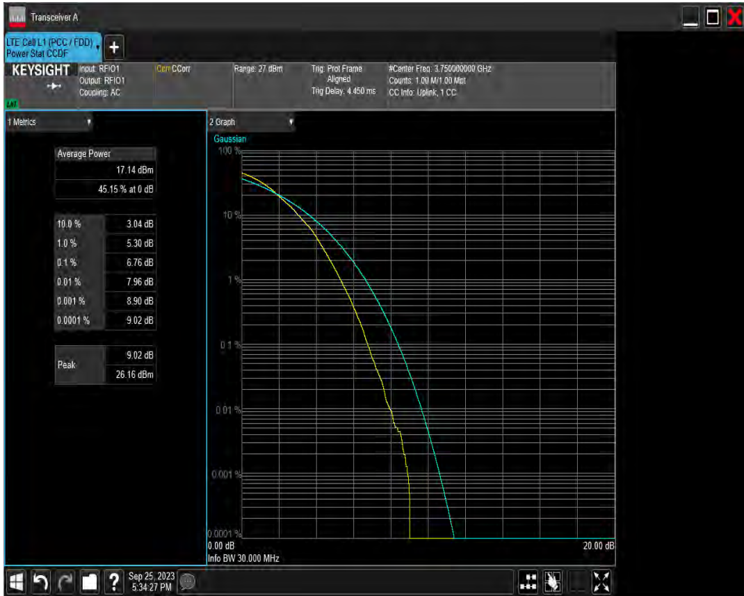
n78(3700-3800) SCS=30kHz DFT 256QAM BW=30MHz Channel=650000 RB=75@0
