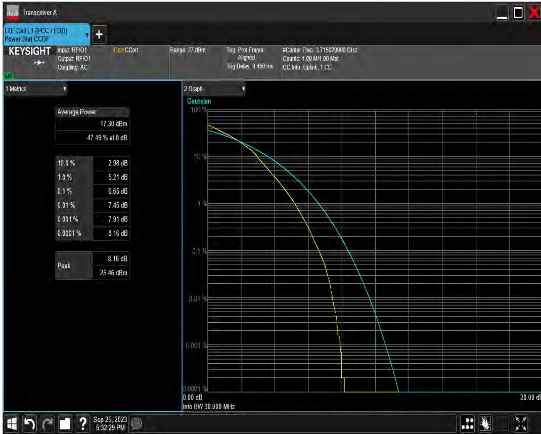
n78(3700-3800) SCS=30kHz DFT 64QAM BW=30MHz Channel=647668 RB=75@0
