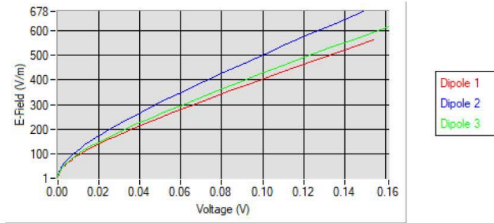
Calibration curves
