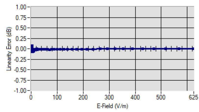
Linearity
