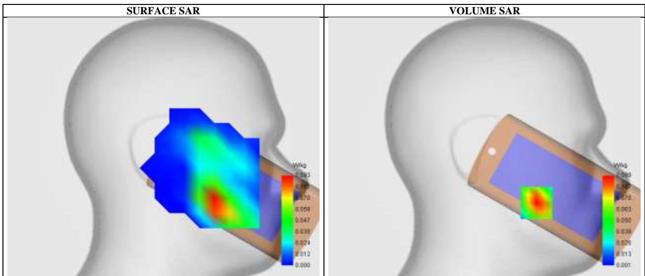
Maximum location: X=-52.00, Y=-56.00 ; SAR Peak: 0.13 W/kg
