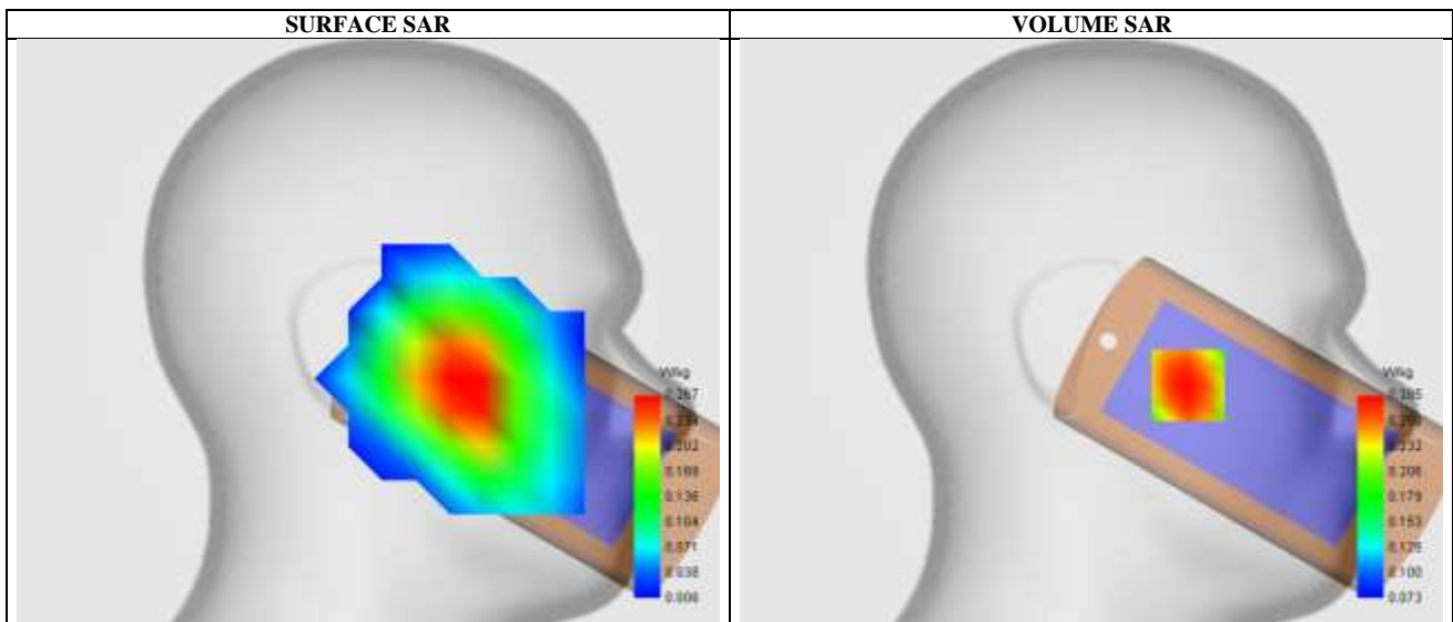
Maximum location: X=-43.00, Y=-24.00 ; SAR Peak: 0.32 W/kg
