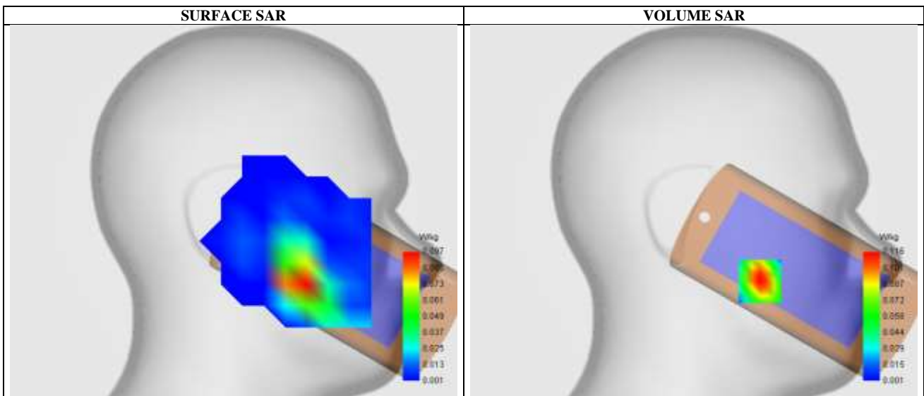
Maximum location: X=-46.00, Y=-49.00 ; SAR Peak: 0.18 W/kg
