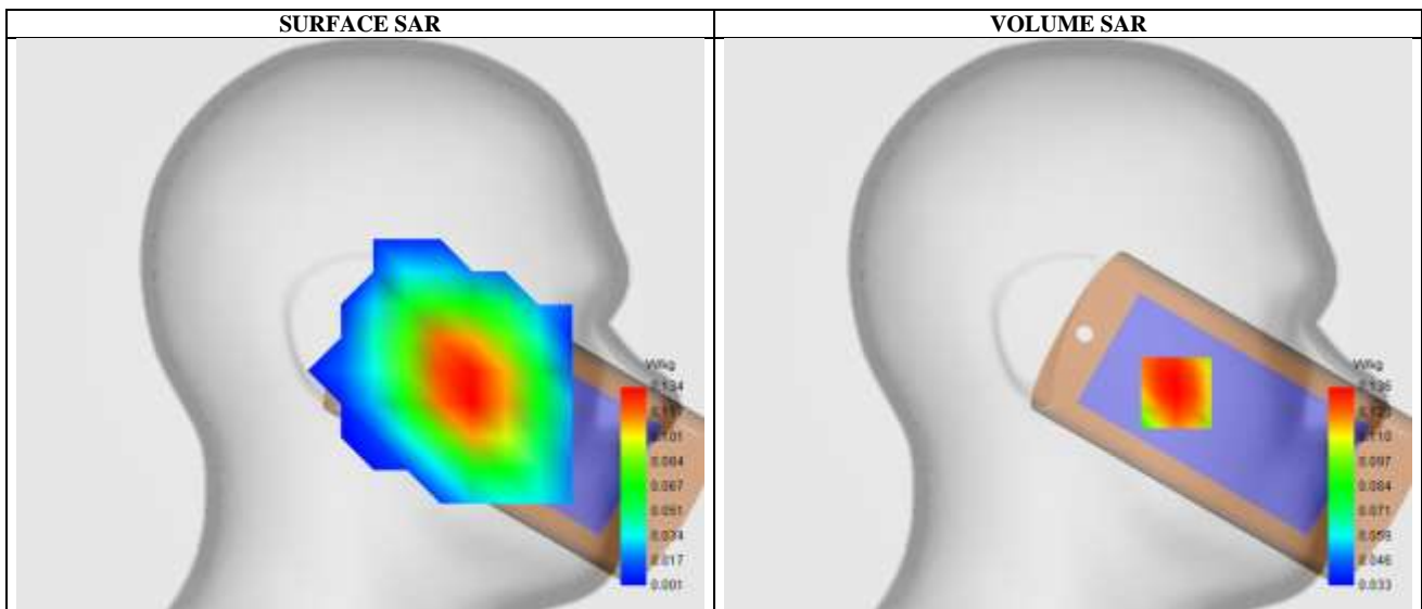
Maximum location: X=-49.00, Y=-31.00 ; SAR Peak: 0.15 W/kg
