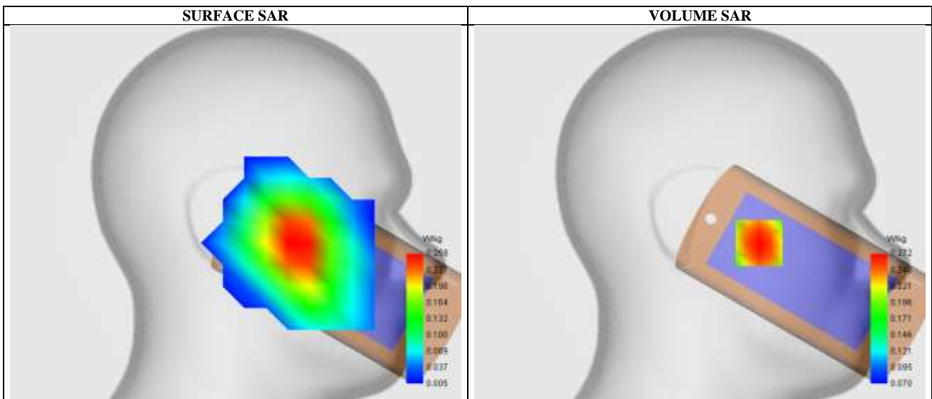
Maximum location: X=-41.00, Y=-21.00 ; SAR Peak: 0.30 W/kg
