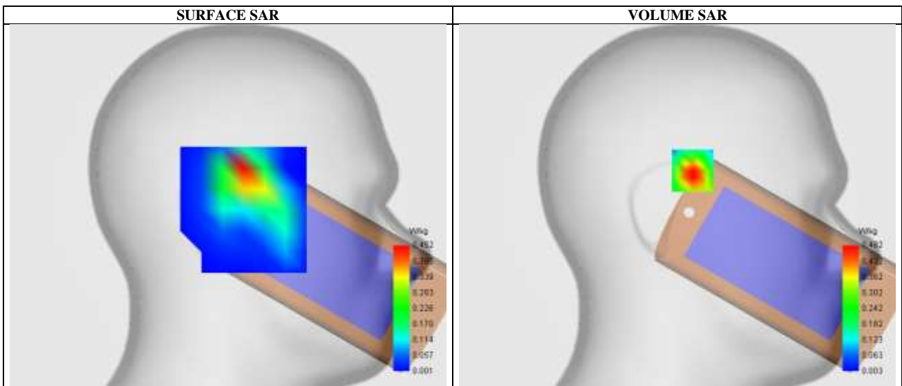
Maximum location: X=-11.00, Y=25.00 ; SAR Peak: 0.83 W/kg
