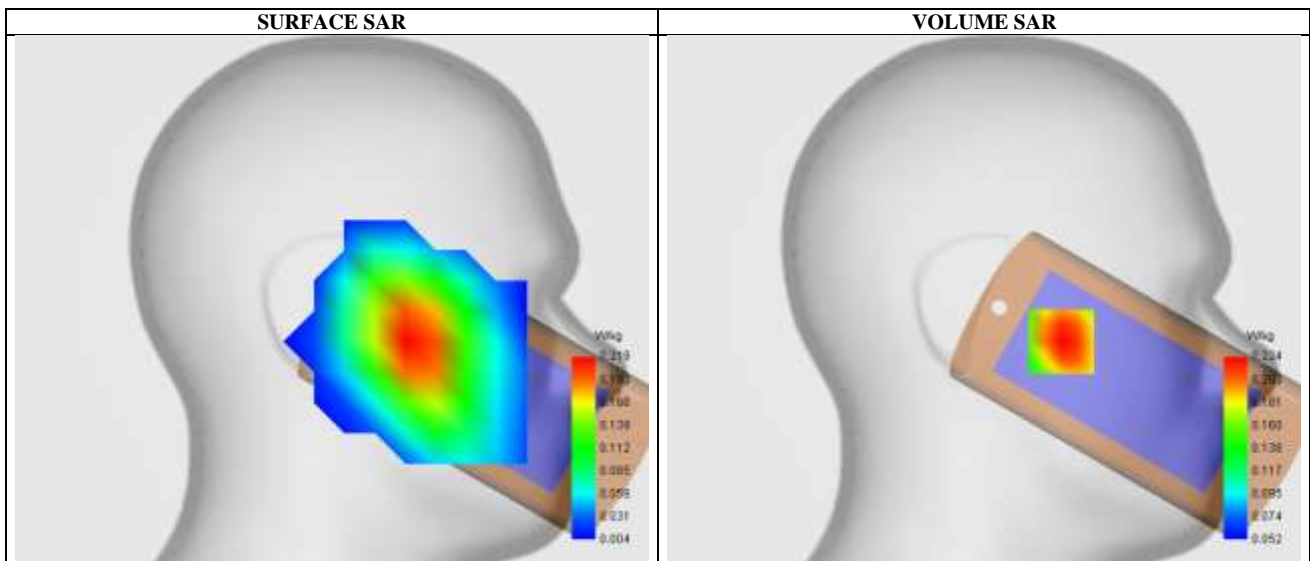
Maximum location: X=-38.00, Y=-21.00 ; SAR Peak: 0.26 W/kg
