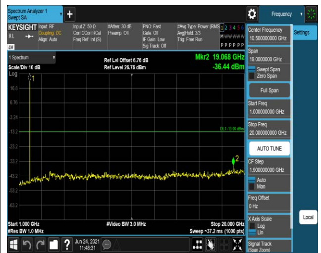
Band25-1.4MHz-16QAM-26683:1000~20000MHz
