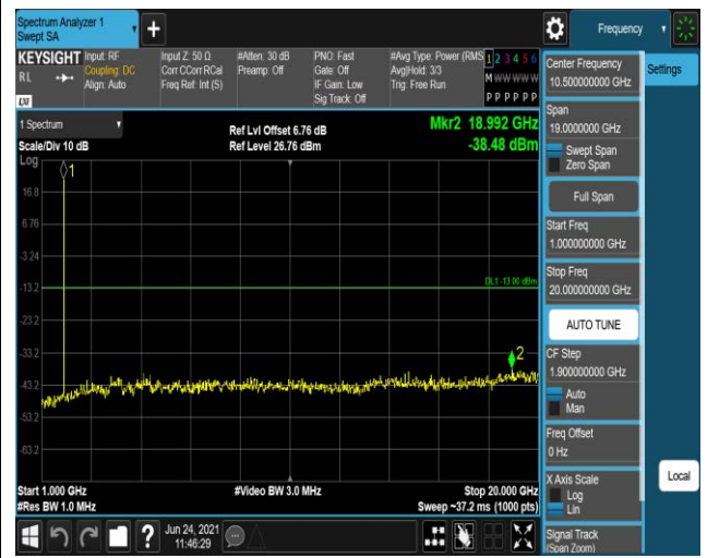
Band25-1.4MHz-16QAM-26365:1000~20000MHz
