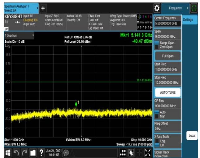
Band12-1.4MHz-16QAM-23095:1000~10000MHz
