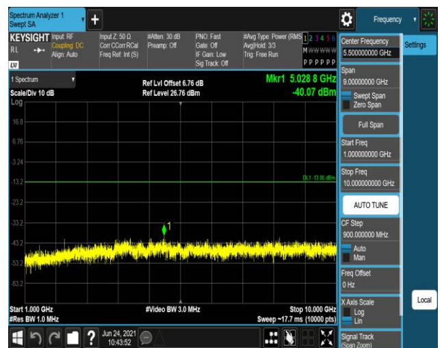
Band12-1.4MHz-16QAM-23173:1000~10000MHz
