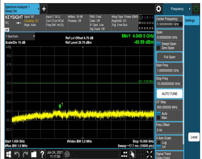
Band12-10MHz-QPSK-23130:1000~10000MHz
