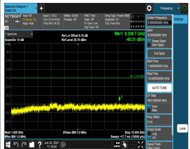
Band12-10MHz-16QAM-23130:1000~10000MHz
