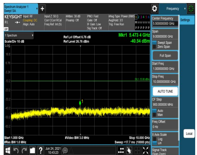
Band12-1.4MHz-QPSK-23173:1000~10000MHz
