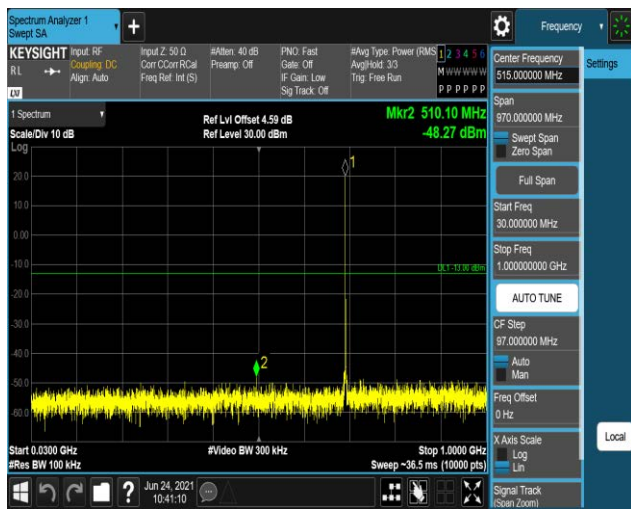
Band12-1.4MHz-QPSK-23095:30~1000MHz
