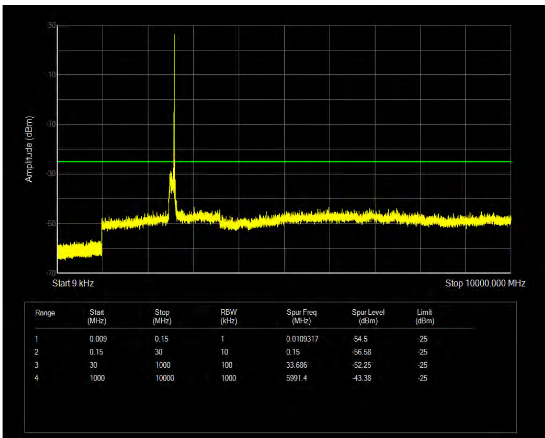
n41 SCS=30kHz CP_QPSK BW=100MHz Channel=518598 RB=273@0
