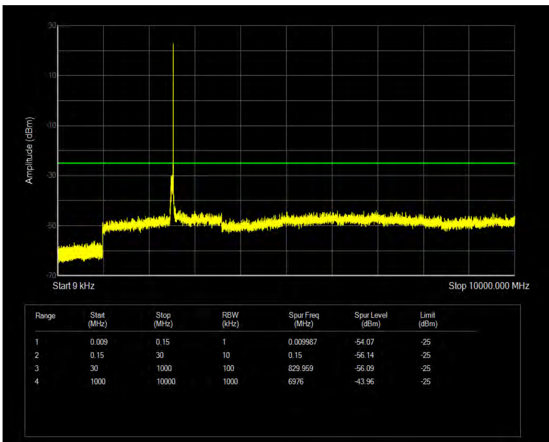
n41 SCS=30kHz CP_QPSK BW=50MHz Channel=518598 RB=133@0
