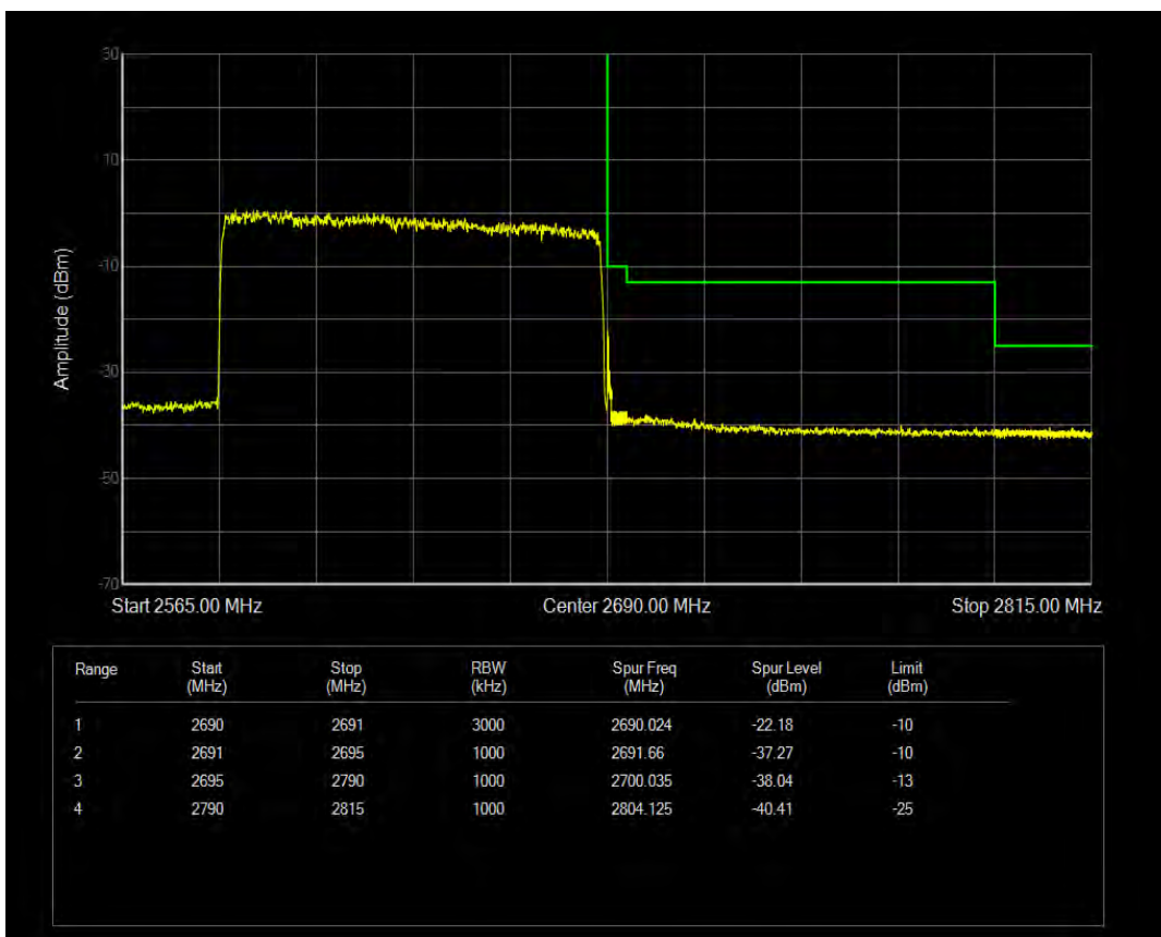
n41 SCS=30kHz DFT_QPSK BW=60MHz Channel=531996 RB=1@161
