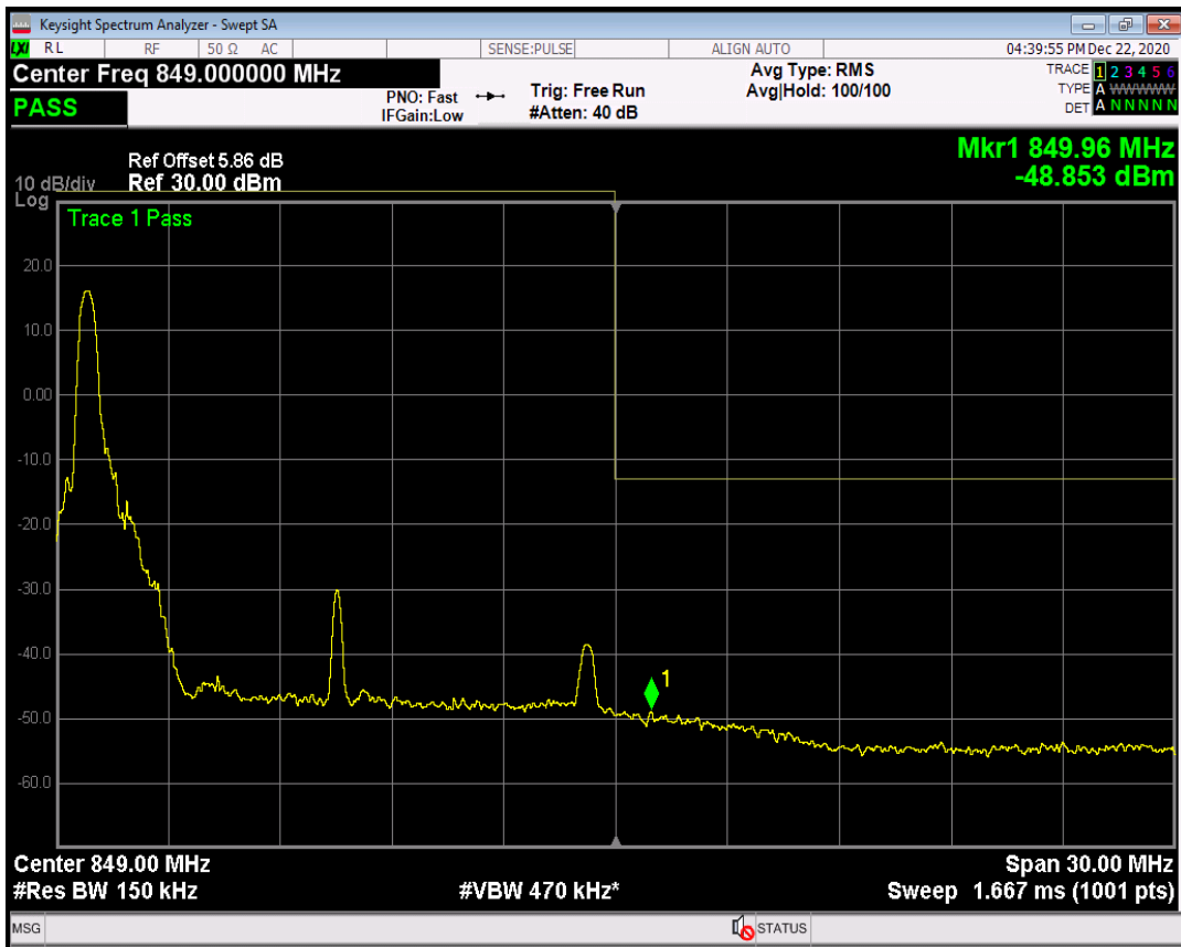
n5 SCS=30kHz CP_QPSK BW=15MHz Channel=168300 RB=1@37
