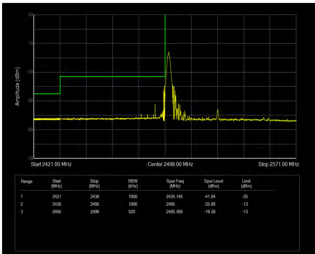
n41 SCS=30kHz CP_QPSK BW=60MHz Channel=505200 RB=1@161
