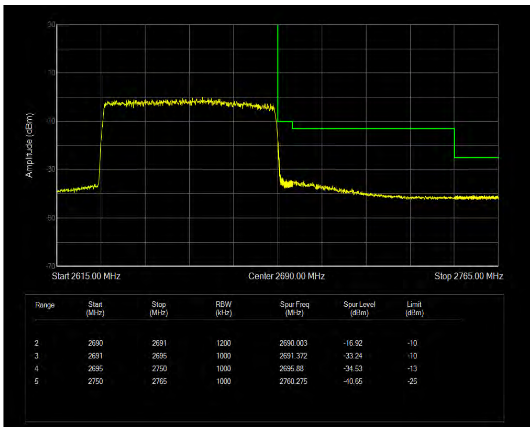
n41 SCS=30kHz CP_QPSK BW=60MHz Channel=531996 RB=1@0
