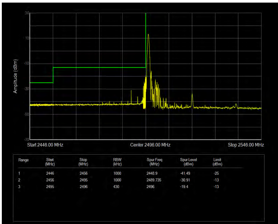
n41 SCS=30kHz CP_QPSK BW=40MHz Channel=503202 RB=1@105
