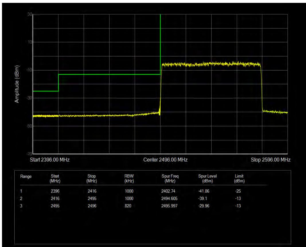
n41 SCS=30kHz CP_QPSK BW=80MHz Channel=507204 RB=1@0
