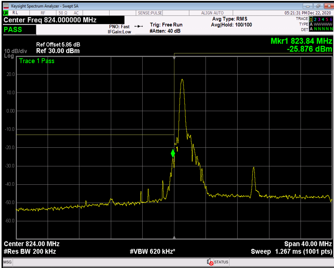
n5 SCS=30kHz CP_QPSK BW=20MHz Channel=166800 RB=1@50
