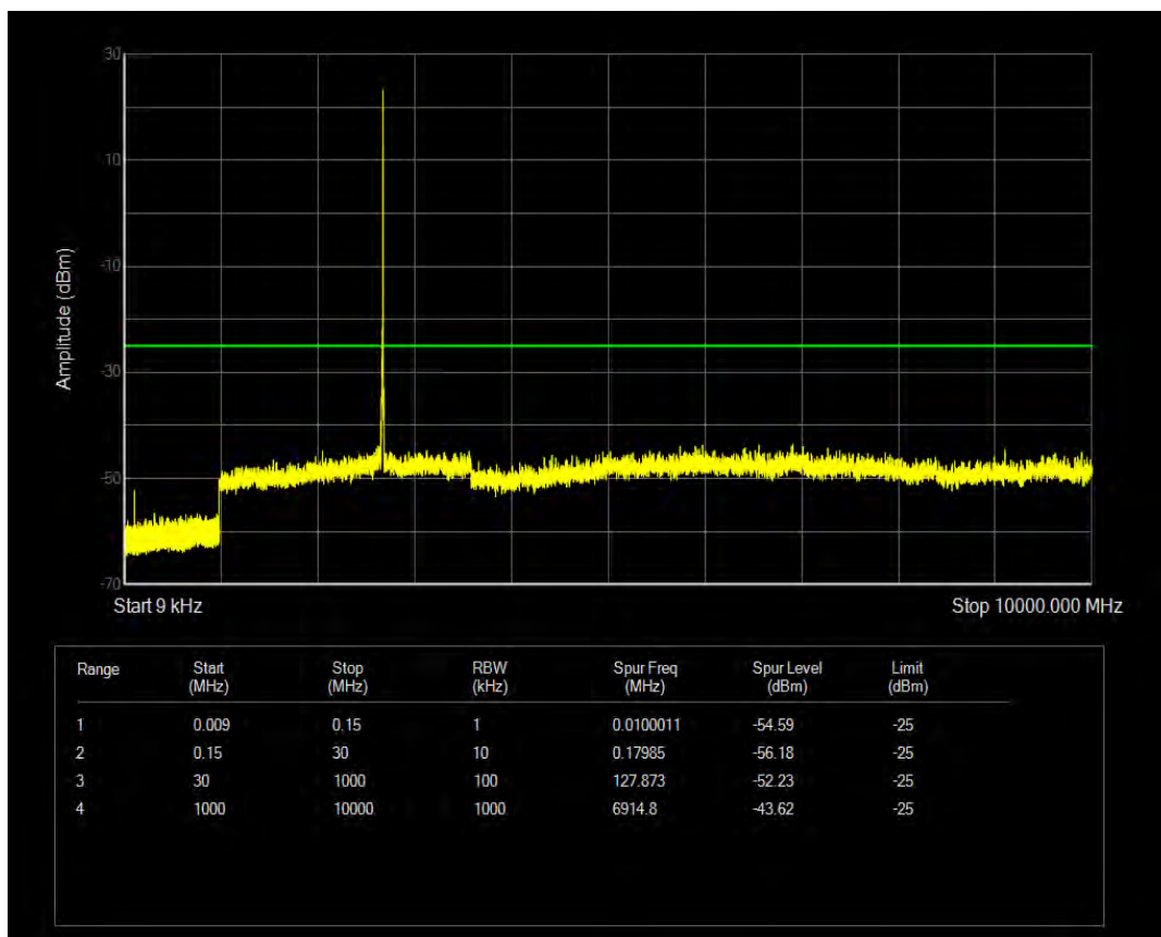
n41 SCS=30kHz CP_QPSK BW=15MHz Channel=500700 RB=36@0
