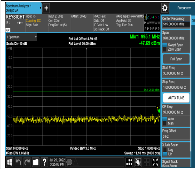
Band7-20MHz-QPSK-21350-1RB#0-Range1:30~1000MHz
