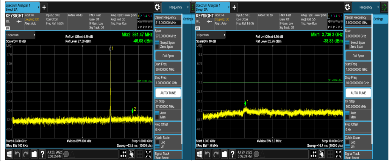
Band 12-1.4MHz-QPSK-23095-1RB#0-Range1:30~1000MHz Band 12-1.4MHz-QPSK-23095-1RB#0-Range2:1000~10000MHz
