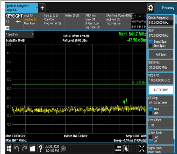
Band7-5MHz-16QAM-20775-1RB#0-Range1:30~1000MHz
