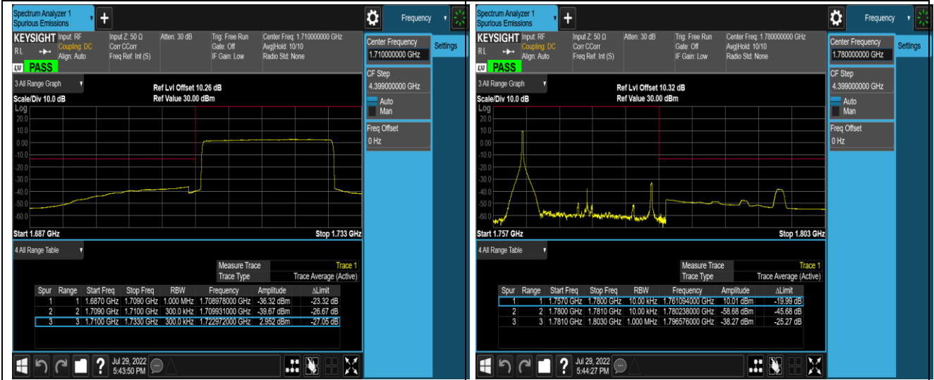
Band66-20MHz-16QAM-132572-1RB#99
