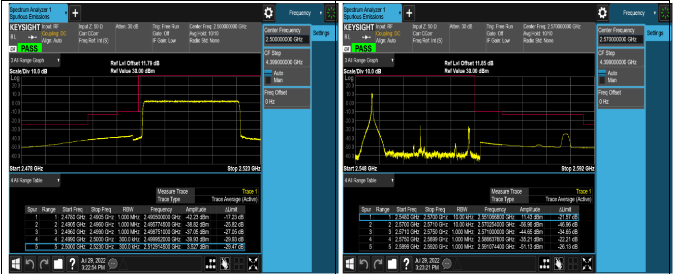
Band7-20MHz-16QAM-21350-1RB#99
