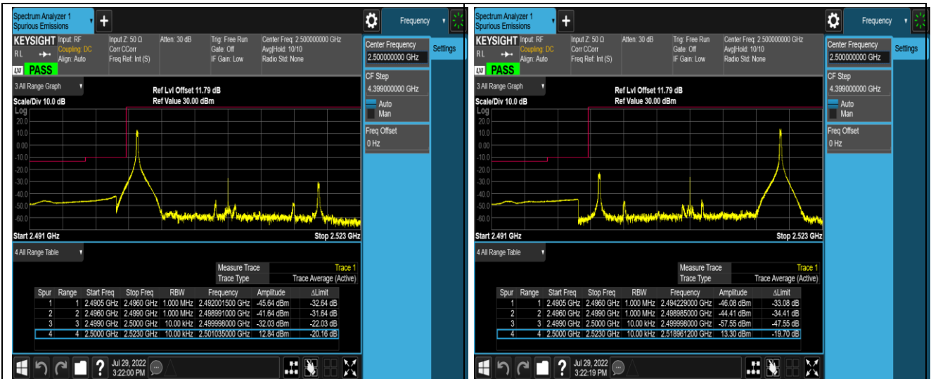
Band7-20MHz-QPSK-20850-100RB#0
