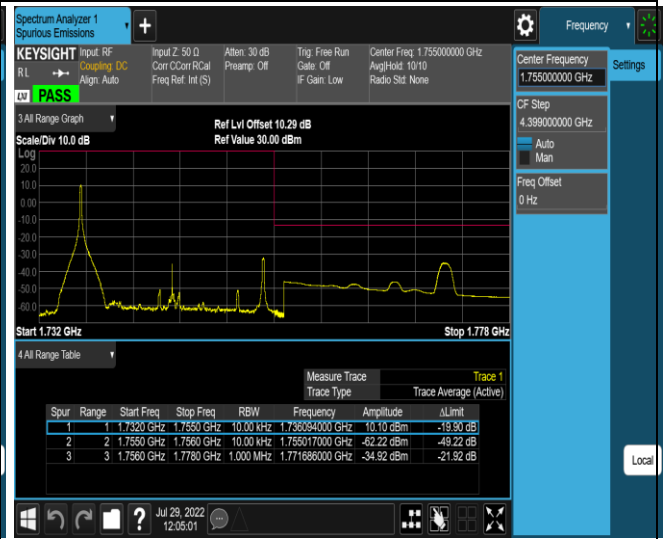
Band4-20MHz-QPSK-20300-100RB#0
