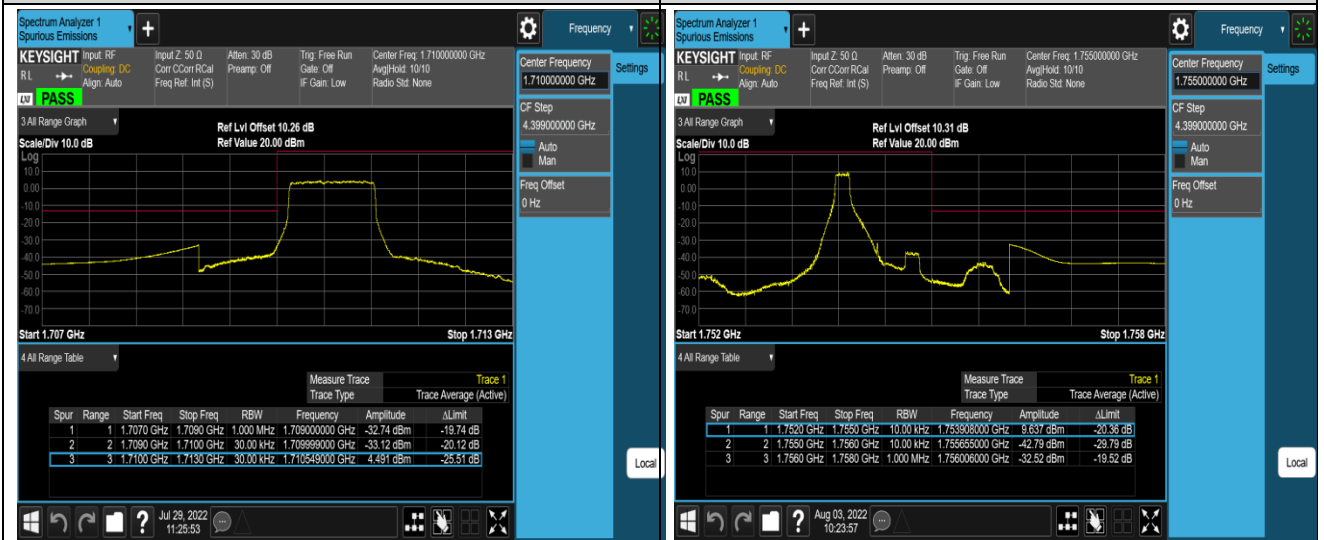
Band4-1.4MHz-16QAM-20393-1RB#5
