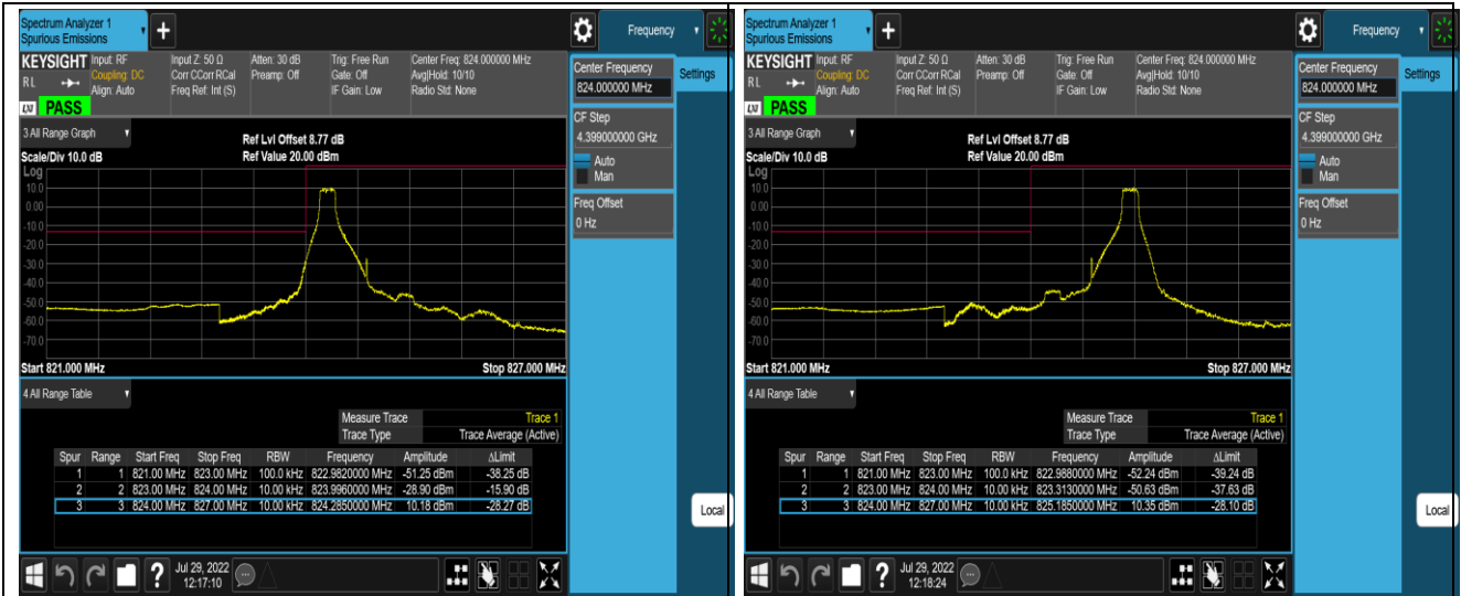
Band5-1.4MHz-QPSK-20407-6RB#0
