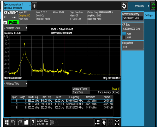
Band5-10MHz-16QAM-20600-50RB#0
