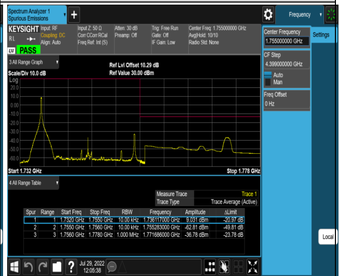
Band4-20MHz-16QAM-20300-100RB#0
