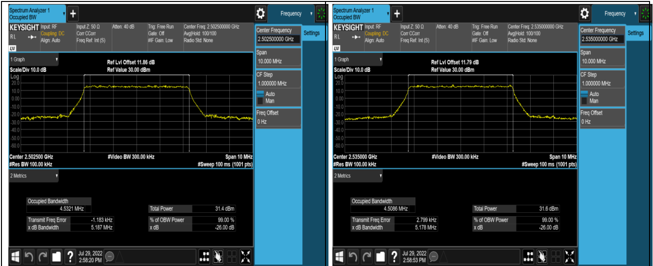
Band7-5MHz-QPSK-21425-25RB#0
