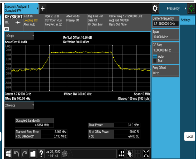
Band4-5MHz-16QAM-20375-25RB#0
