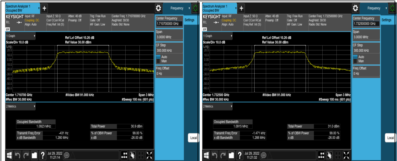
Band4-1.4MHz-QPSK-20393-6RB#0
