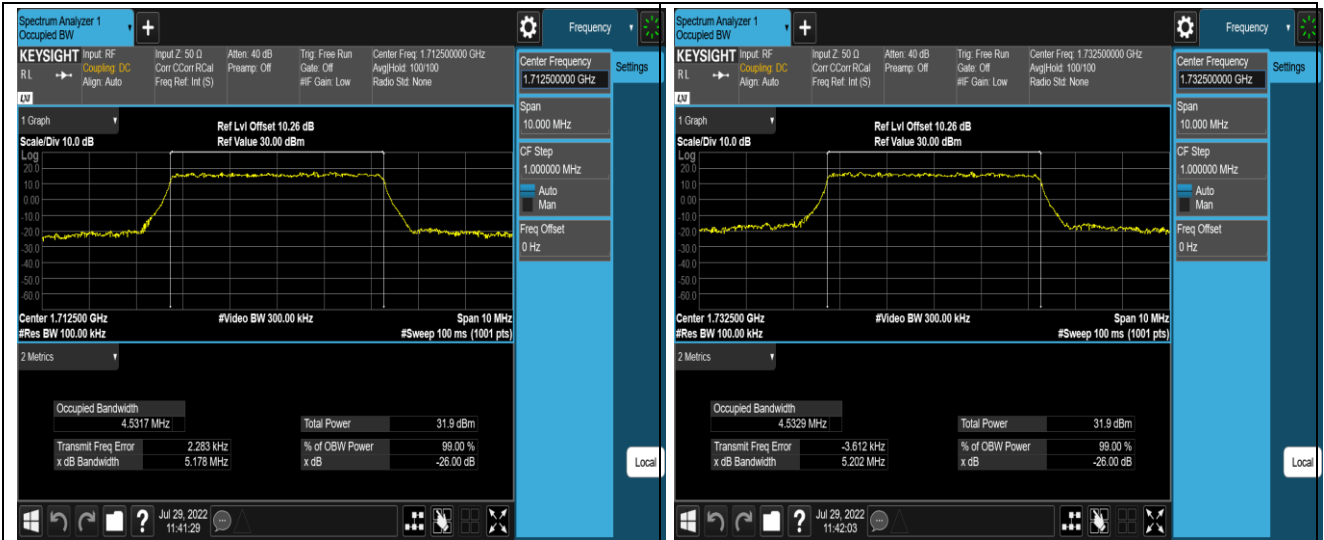
Band4-5MHz-QPSK-20375-25RB#0
