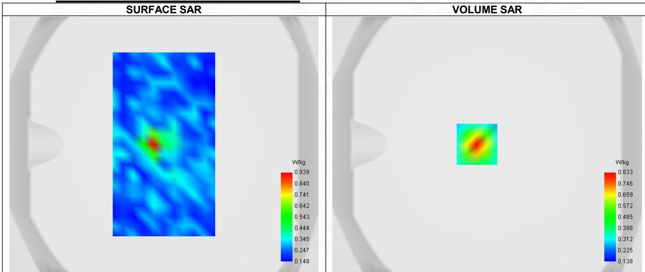
Maximum location: X=-8.00, Y=0.00 ; SAR Peak: 1.25 W/kg
