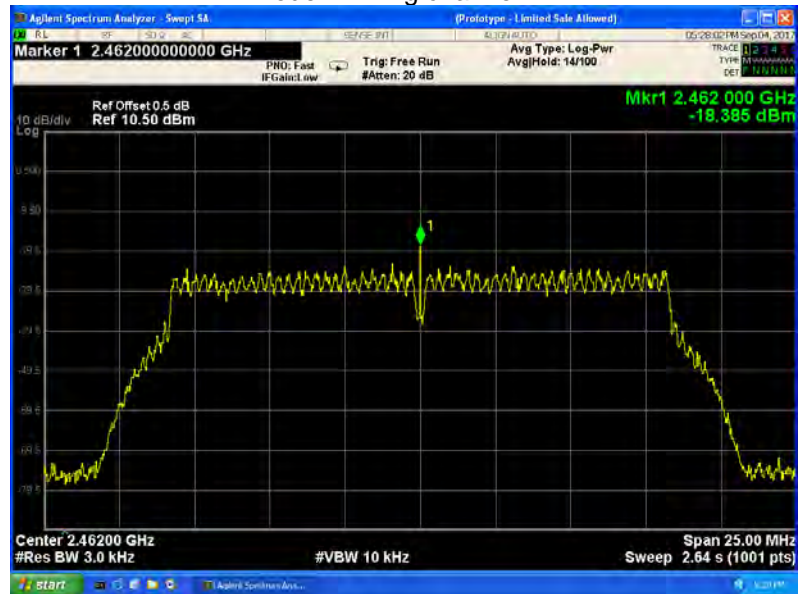
Mode :TX 11g channel 11
