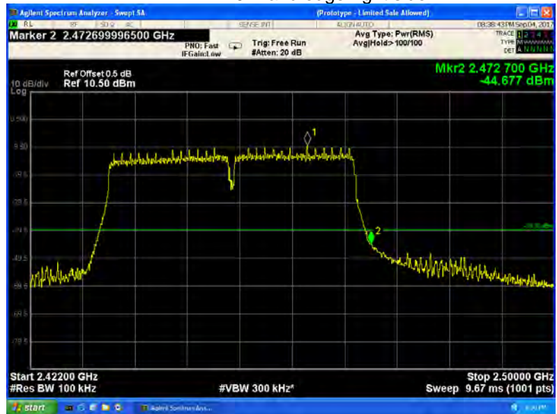
TX 11n HT40: Band edge-right side
