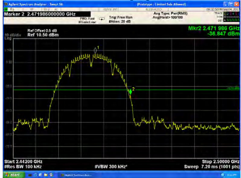
TX 11b: Band edge-right side
