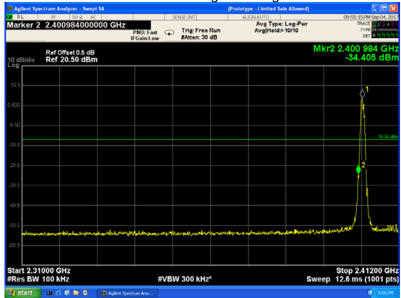
GFSK Transmitting Band edge-left side
