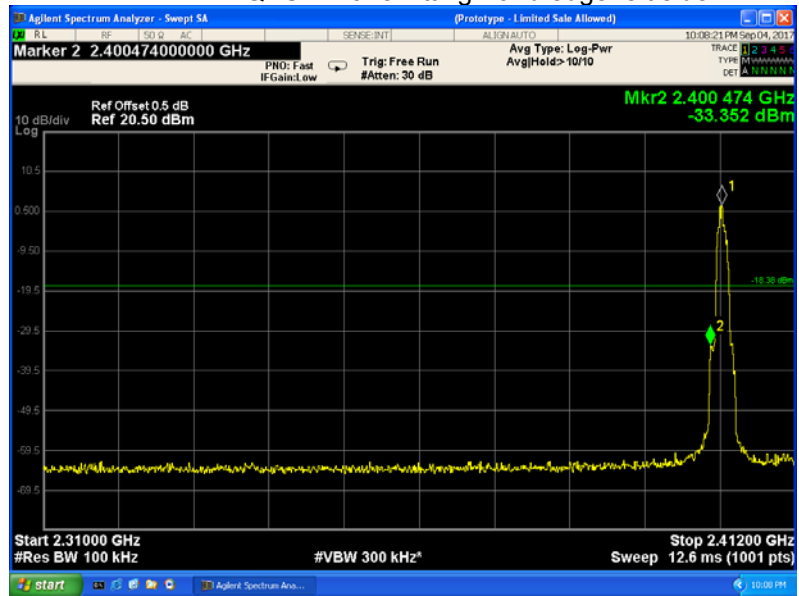
Pi/4 DQPSK Transmitting Band edge-left side
