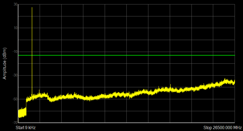
Band66 16QAM BW=3MHz Channel=131987 RB Size=1 Position=#0
