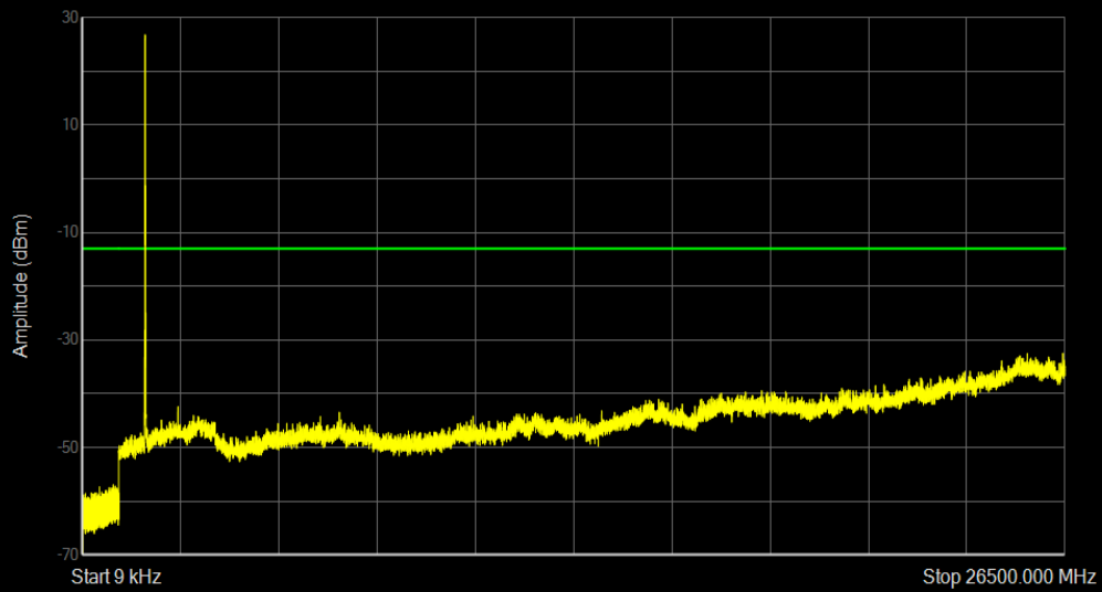
Band66 16QAM BW=10MHz Channel=132022 RB Size=1 Position=#0
