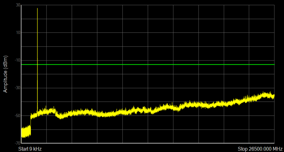
Band66 16QAM BW=5MHz Channel=131997 RB Size=1 Position=#0
