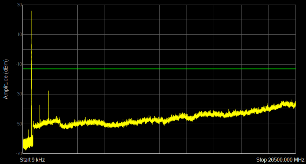
Band26(824-849) QPSK BW=15MHz Channel=26915 RB Size=1 Position=#0
