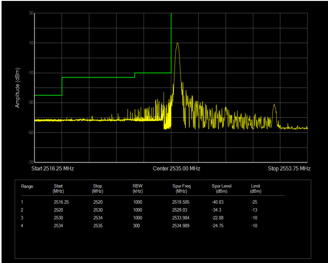
Band41(2535-2655) 16QAM BW=15MHz Channel=40115 RB Size=1 Position=#Max
