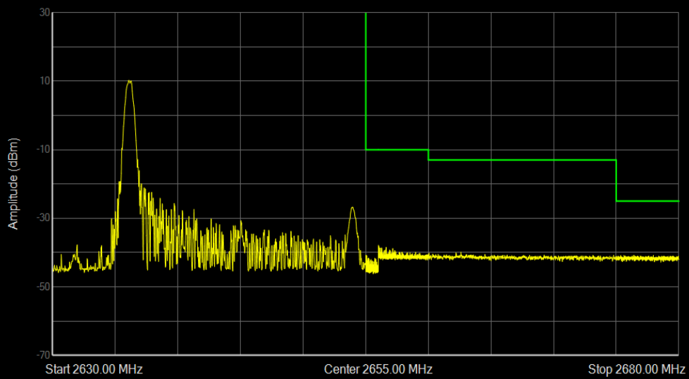
Band41(2535-2655) QPSK BW=20MHz Channel=41140 RB Size=1 Position=#0
