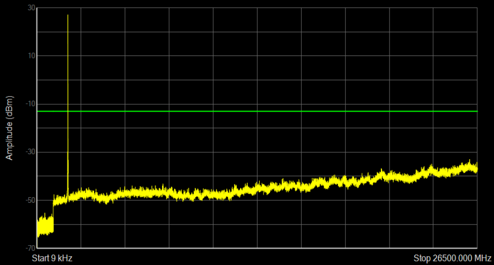
Band25 16QAM BW=10MHz Channel=26365 RB Size=1 Position=#0
