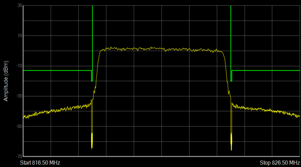
Band26a 16QAM BW=5MHz Channel=26765 RB Size=25 Position=#0
