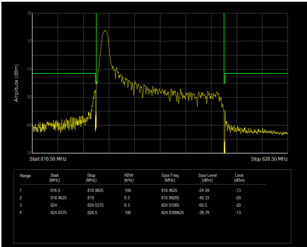
Band26a 16QAM BW=5MHz Channel=26765 RB Size=1 Position=#Max
