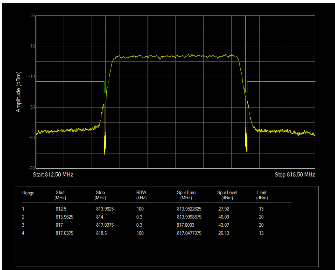
Band26a 16QAM BW=3MHz Channel=26705 RB Size=1 Position=#Max
