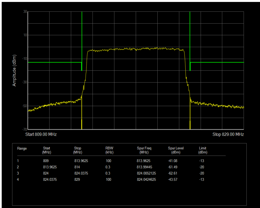
Band26a 16QAM BW=10MHz Channel=26740 RB Size=1 Position=#Max
