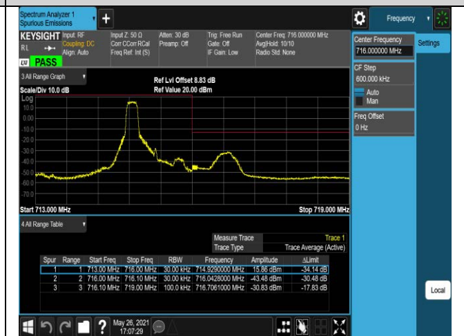
Band12-1.4MHz-QPSK-23173-6RB#0
