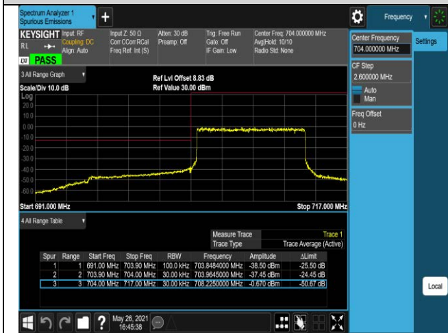
Band17-10MHz-QPSK-23800-1RB#49
