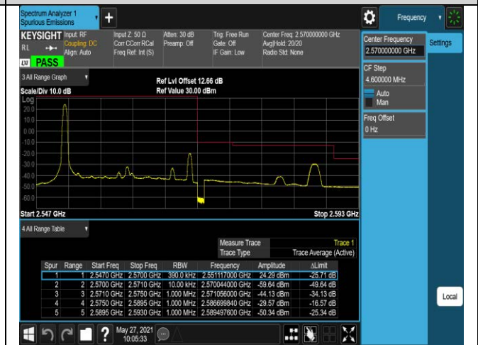
Band7-20MHz-QPSK-21350-100RB#0
