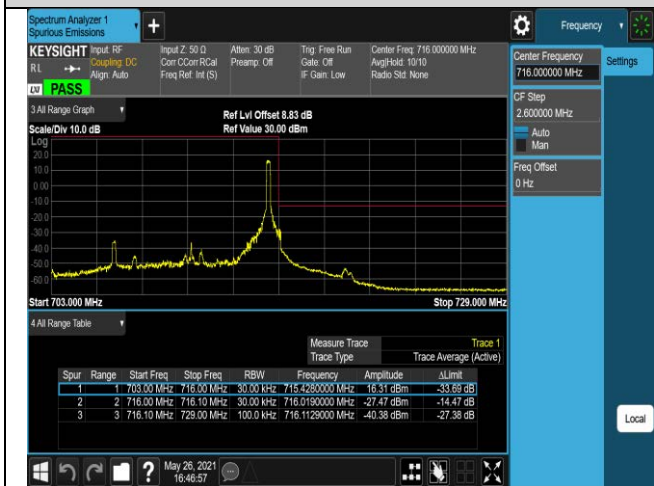
Band17-10MHz-16QAM-23780-1RB#0
