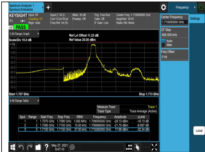
Band4-1.4MHz-QPSK-19957-6RB#0
