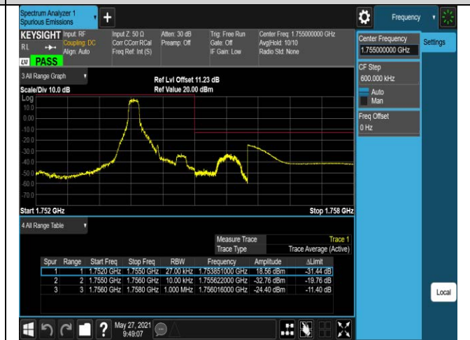
Band4-1.4MHz-QPSK-20393-6RB#0
