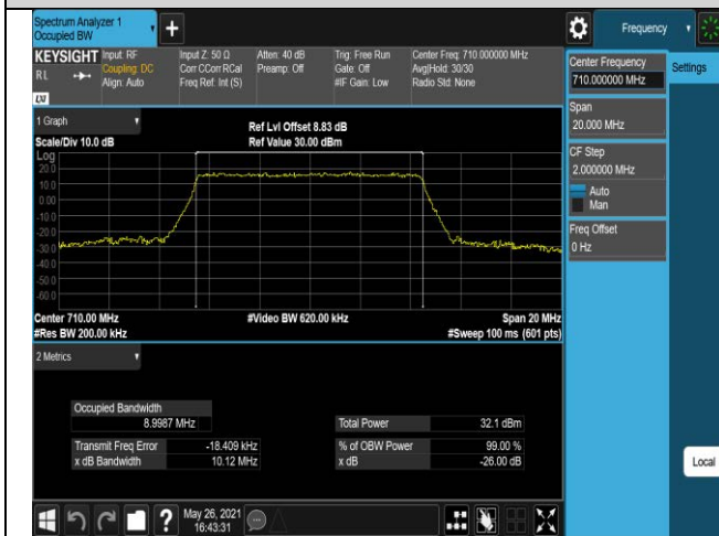
Band17-10MHz-16QAM-23790-50RB#0
