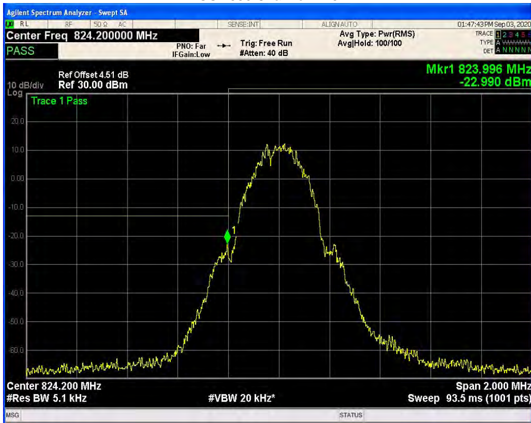
GSM850 Channel=128
