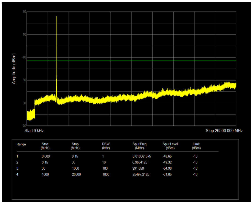
n78 SCS=30kHz CP_QPSK BW=60MHz Channel=651332 RB=1@161
