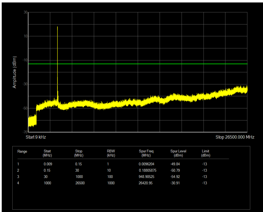
n78 SCS=30kHz CP_QPSK BW=10MHz Channel=636666 RB=1@0
