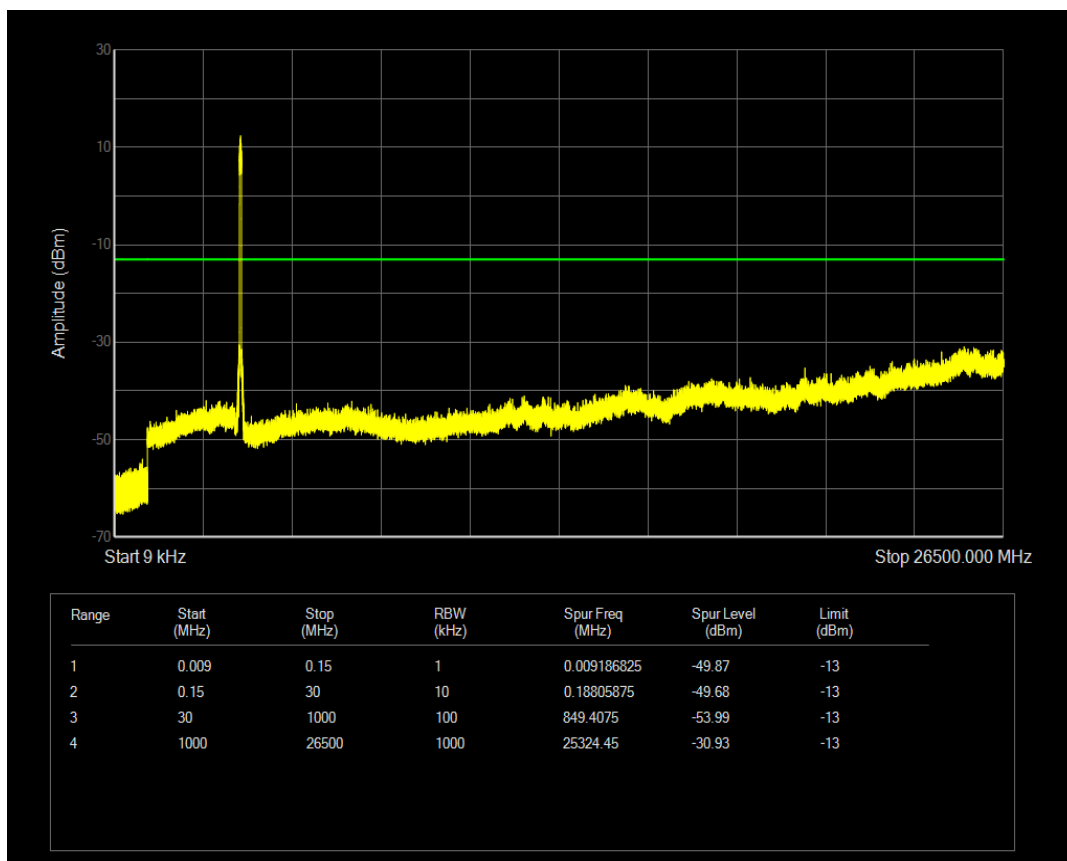
n78 SCS=30kHz CP_QPSK BW=60MHz Channel=651332 RB=1@0
