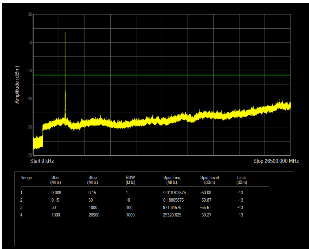
n78 SCS=30kHz CP_QPSK BW=15MHz Channel=620500 RB=1@0
