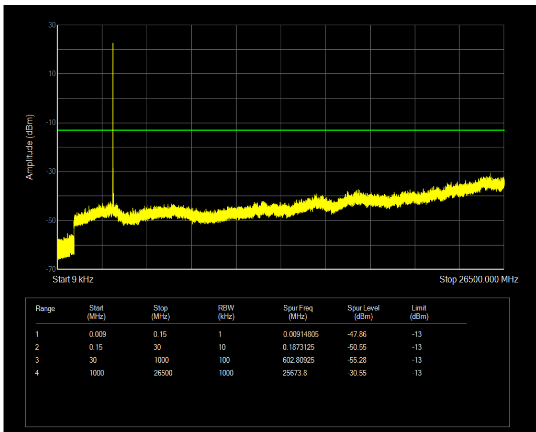
n78 SCS=30kHz CP_QPSK BW=15MHz Channel=620500 RB=1@37
