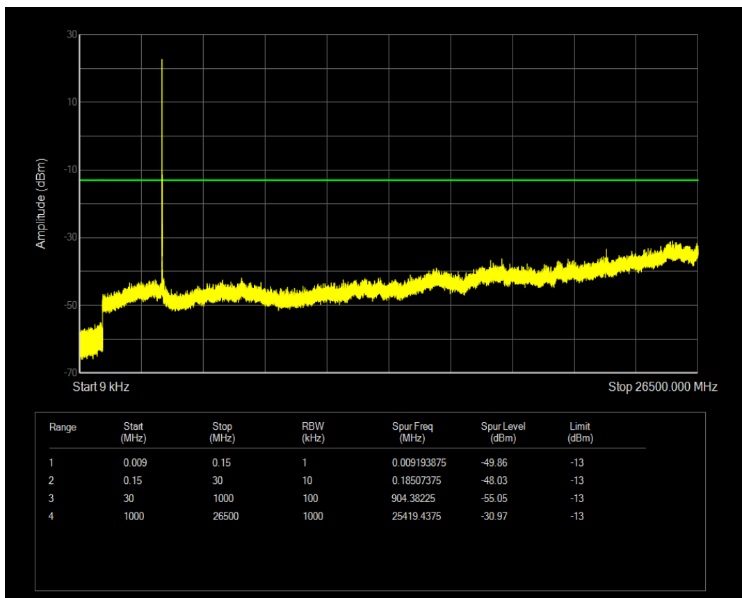
n78 SCS=30kHz CP_QPSK BW=10MHz Channel=636666 RB=1@23
