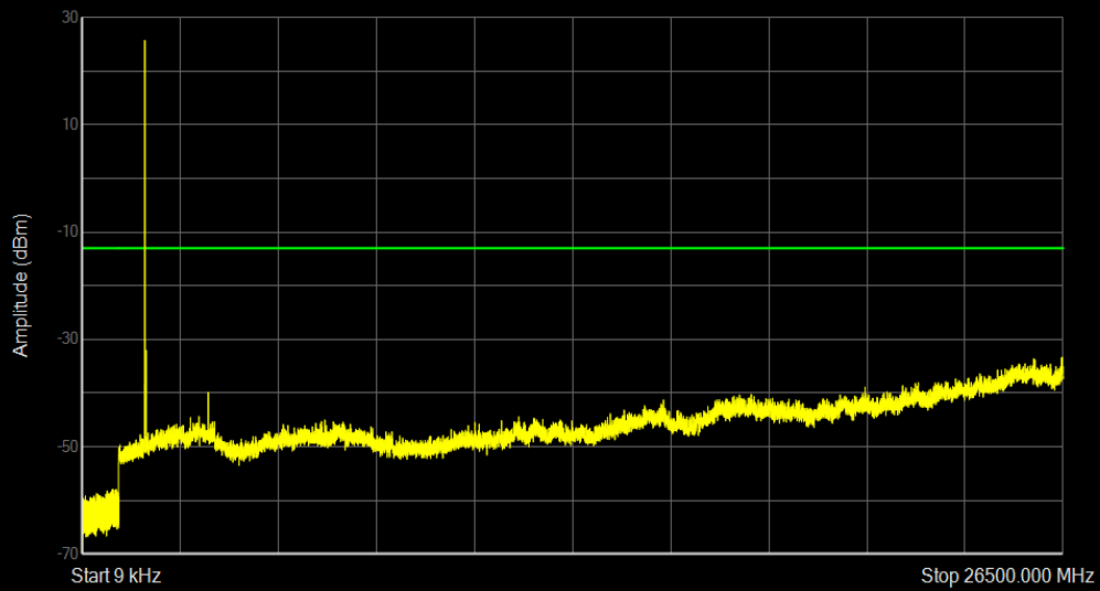
Band4 16QAM BW=1.4MHz Channel=19957 RB Size=1 Position=#0
