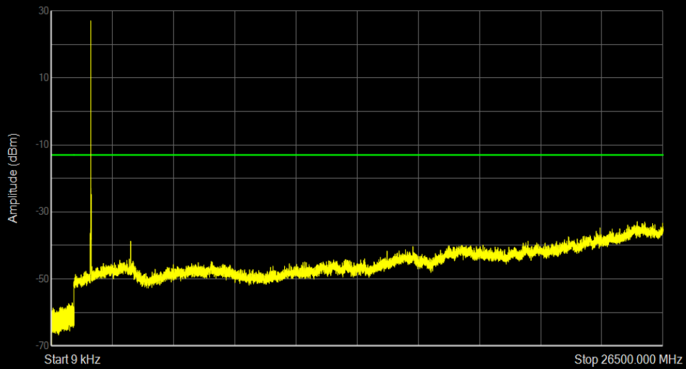
Band4 16QAM BW=10MHz Channel=20175 RB Size=1 Position=#0
