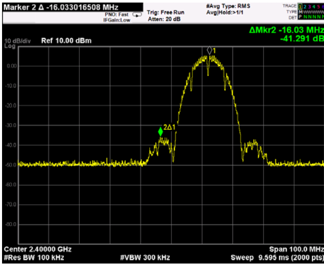
802.11g_CH Low
