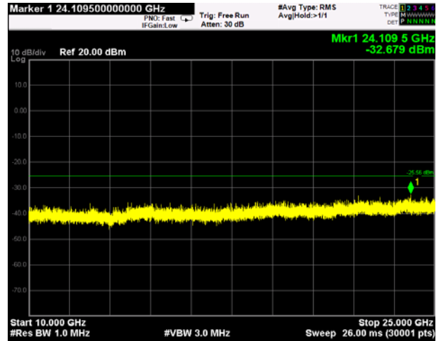
802.11b_CH Middle(Above 1 GHz)
