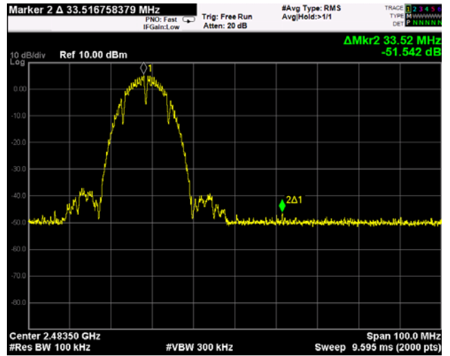
802.11g_CH High
