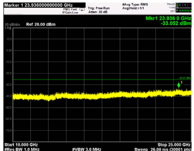
802.11b_CH High(Above 1 GHz)
