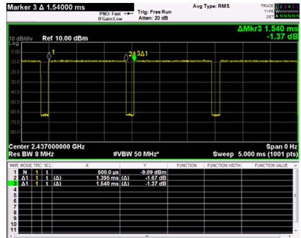
802.11n_HT40(MCS0)
