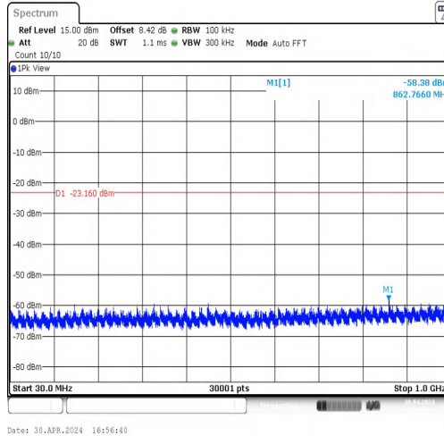
11B-CDD-Ant2-2462-30~1000-PASS
