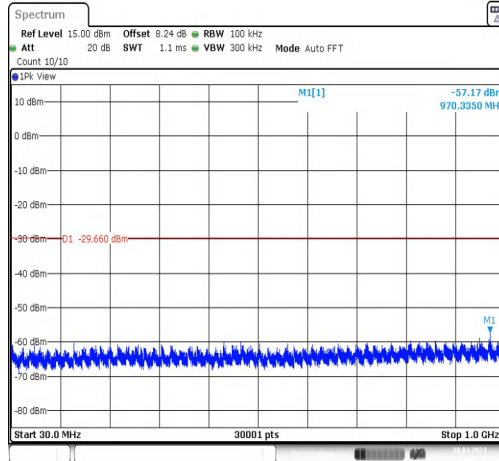
11N40MIMO-Ant2-2422-0~Reference-PASS
