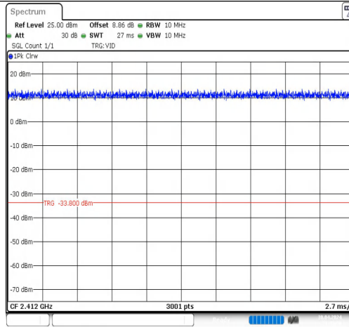
NTNV-11N20MIMO-Ant1-2412
