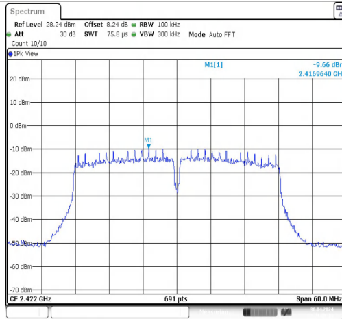
11N40MIMO-Ant2-2422-0~Reference-PASS
