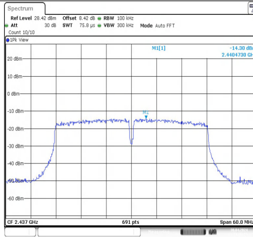
11N40MIMO-Ant2-2437-0~Reference-PASS
