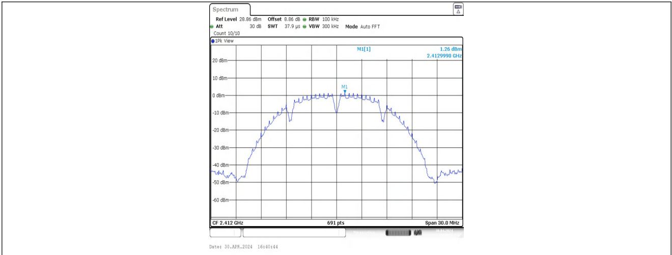
11B-CDD-Ant1-2412-0~Reference-PASS
