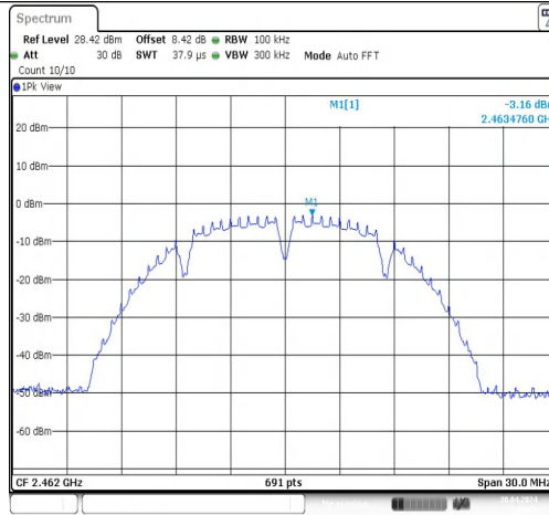
11B-CDD-Ant2-2462-0~Reference-PASS
