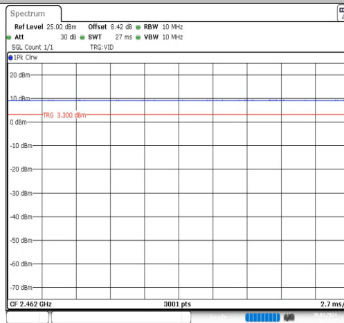
NTNV-11B-CDD-Ant1-2462
