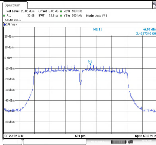
11N40MIMO-Ant1-2422-0~Reference-PASS
