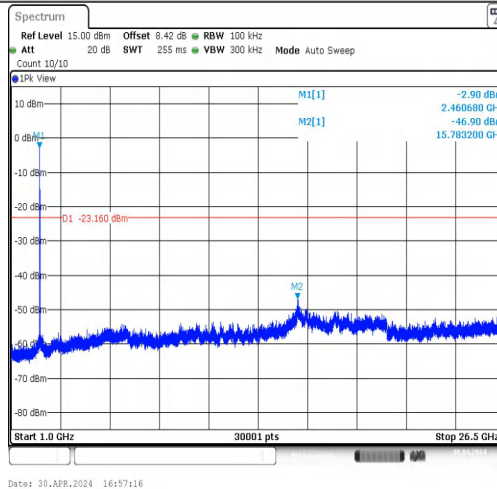
11B-CDD-Ant2-2462-1000~26500-PASS
