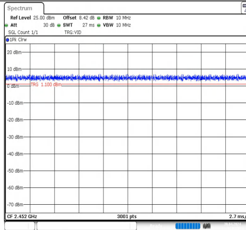
NTNV-11N40MIMO-Ant1-2452
