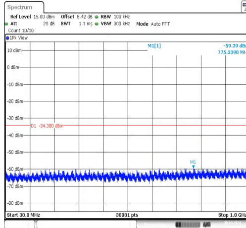
11N40MIMO-Ant2-2437-0~Reference-PASS
