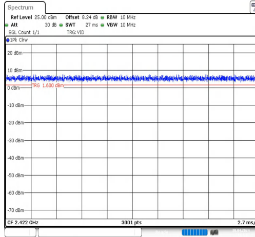
NTNV-11N40MIMO-Ant1-2422
