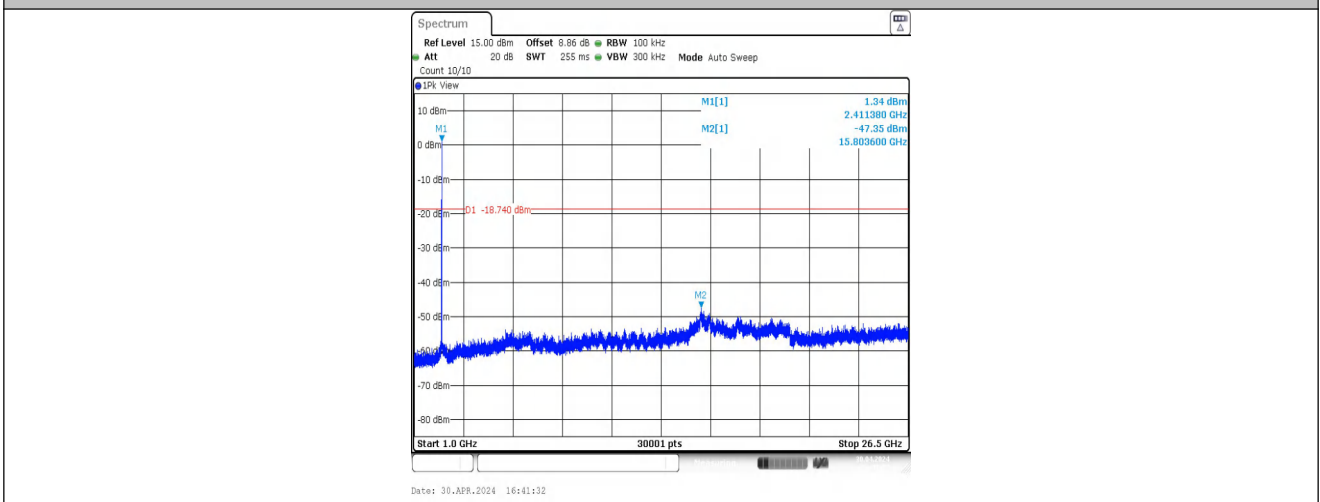
11B-CDD-Ant1-2412-1000~26500-PASS
