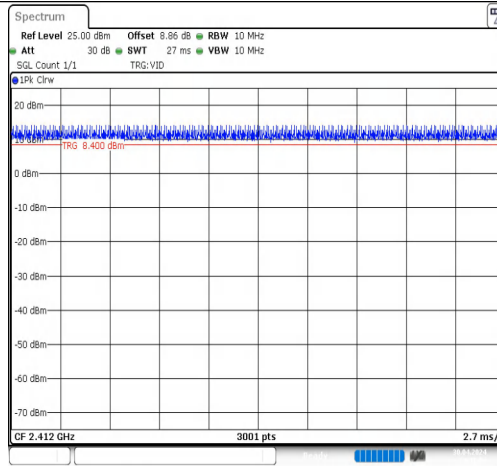
NTNV-11G-CDD-Ant1-2412
