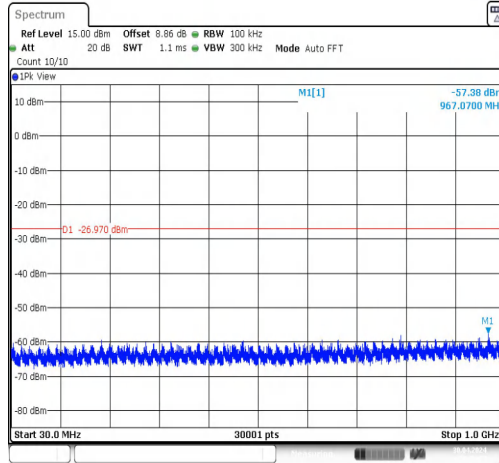
11N40MIMO-Ant1-2422-0~Reference-PASS
