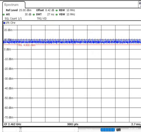
NTNV-11G-CDD-Ant1-2462
