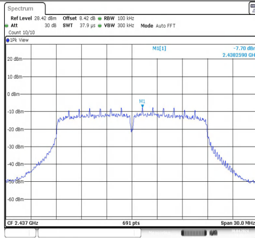
11N20MIMO-Ant2-2437-0~Reference-PASS
