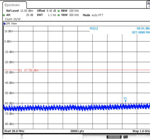
11N20MIMO-Ant2-2437-0~Reference-PASS
