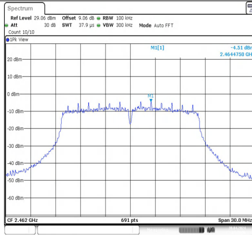
11G-CDD-Ant1-2462-0~Reference-PASS
