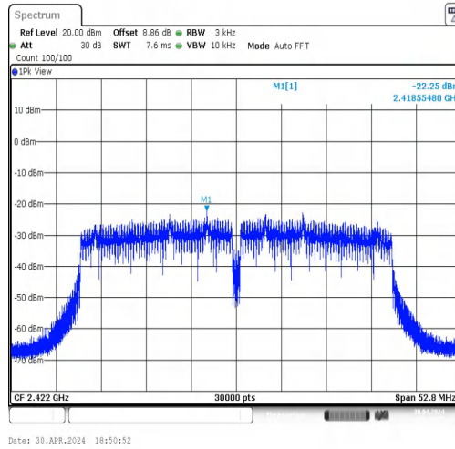
11N40MIMO-Ant1-2422-PASS
