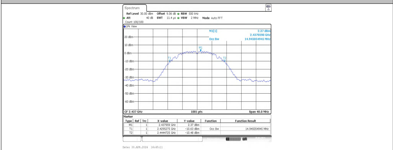
11B-CDD-Ant1-2437
