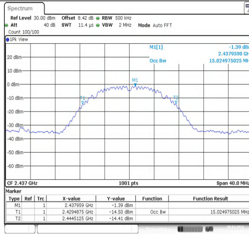
11B-CDD-Ant2-2437
