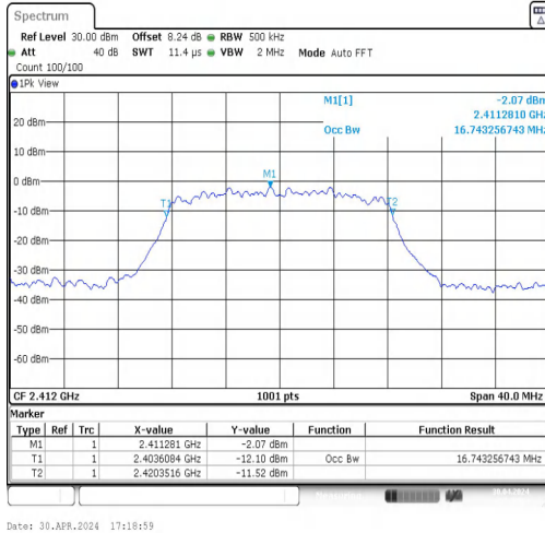
11G-CDD-Ant2-2412
