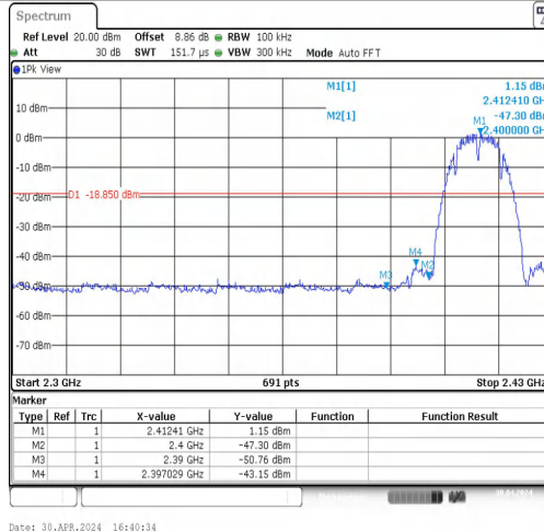
11B-CDD-Ant1-2412-PASS
