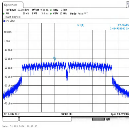
11G-CDD-Ant1-2437-PASS
