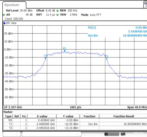
11G-CDD-Ant2-2437
