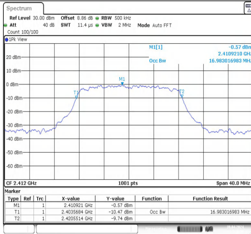
11G-CDD-Ant1-2412
