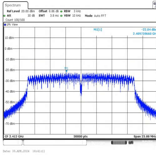
11G-CDD-Ant1-2412-PASS
