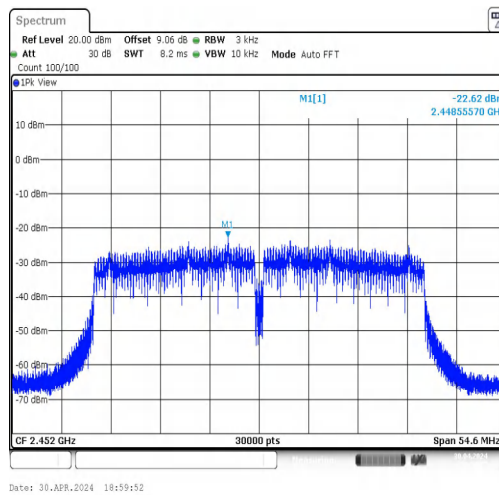
11N40MIMO-Ant1-2452-PASS
