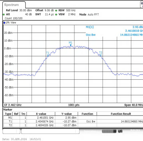
11B-CDD-Ant1-2462
