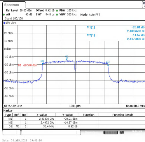
11N40MIMO-Ant2-2452-PASS
