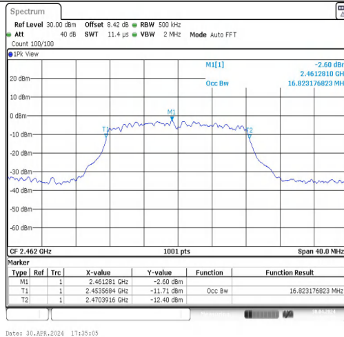
11G-CDD-Ant2-2462
