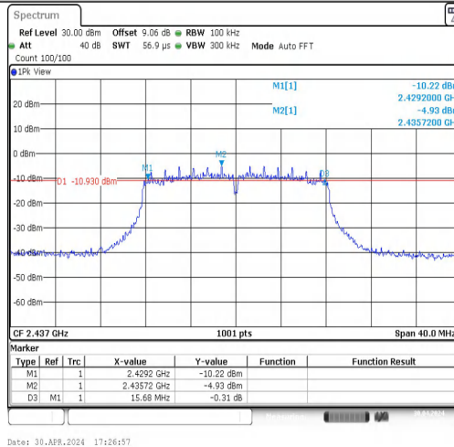
11G-CDD-Ant1-2437-PASS
