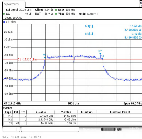
11G-CDD-Ant2-2412-PASS
