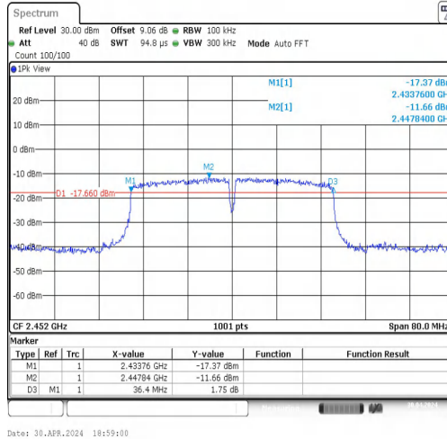
11N40MIMO-Ant1-2452-PASS
