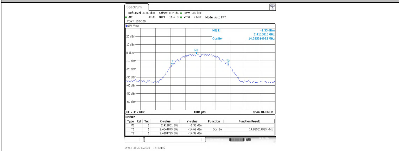
11B-CDD-Ant2-2412
