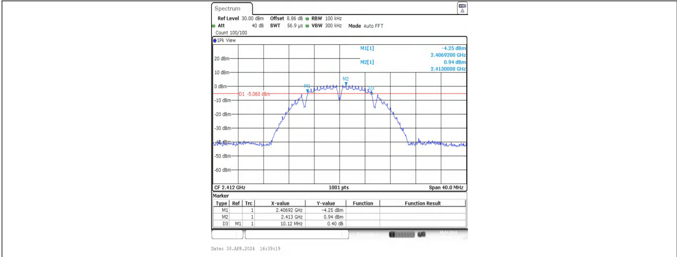
11B-CDD-Ant1-2412-PASS
