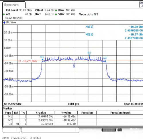
11N40MIMO-Ant2-2422-PASS
