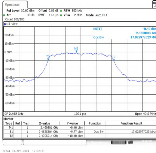
11G-CDD-Ant1-2462
