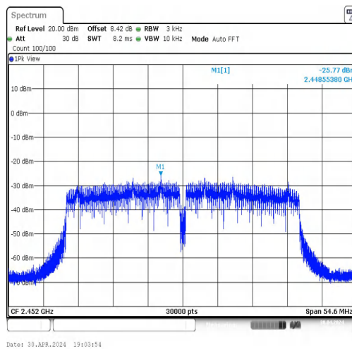
11N40MIMO-Ant2-2452-PASS
