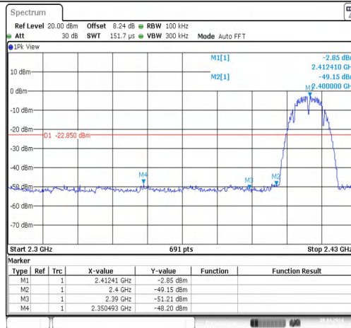
11B-CDD-Ant1-2412-PASS
