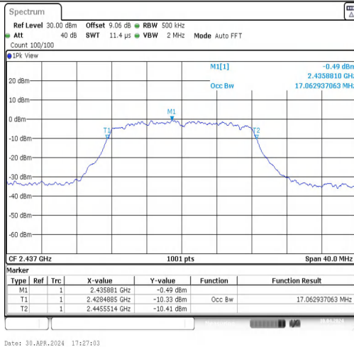
11G-CDD-Ant1-2437
