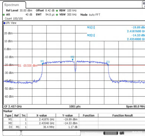
11N40MIMO-Ant2-2437-PASS
