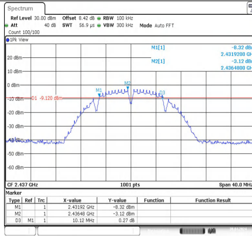
11B-CDD-Ant2-2437-PASS
