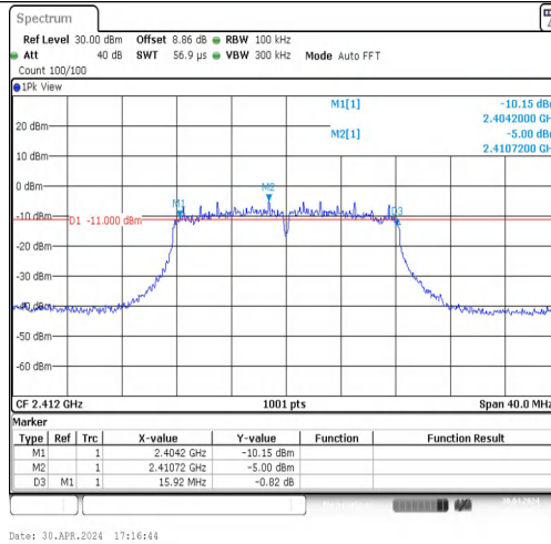
11G-CDD-Ant1-2412-PASS
