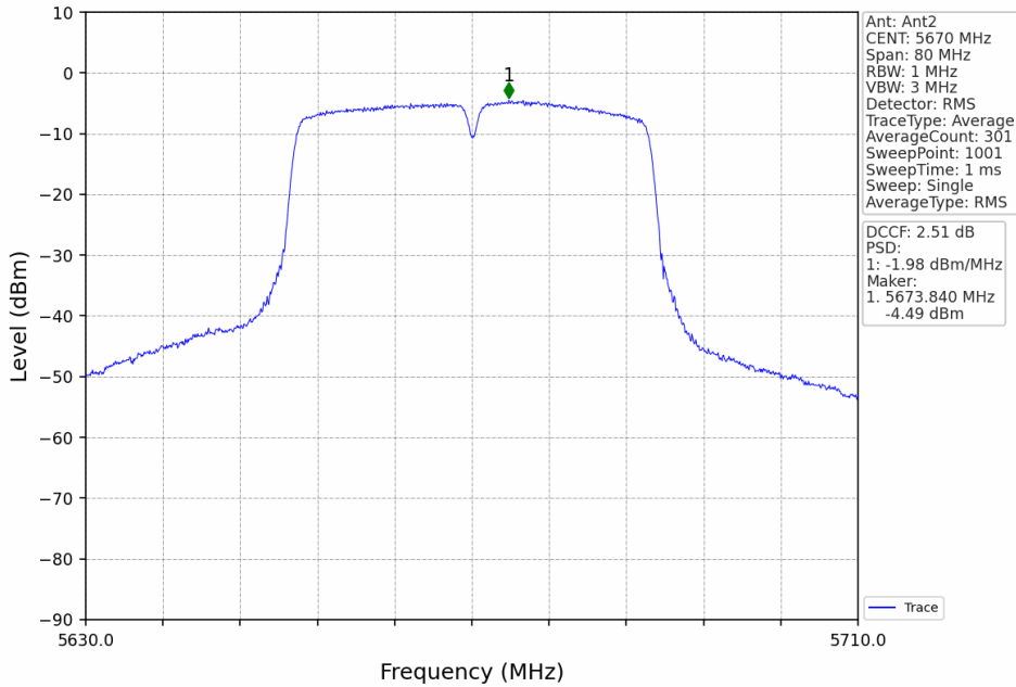
802.11ac(VHT40)_HCH_5670MHz_MIMO_NTNV
