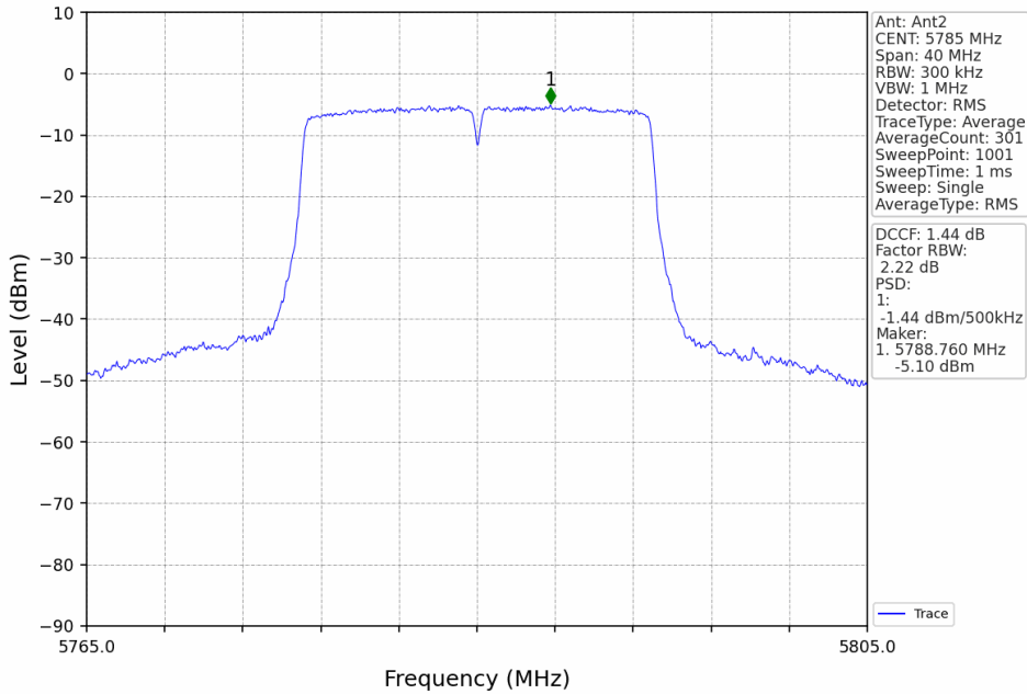
802.11ac(VHT20)_MCH_5785MHz_MIMO_NTNV
