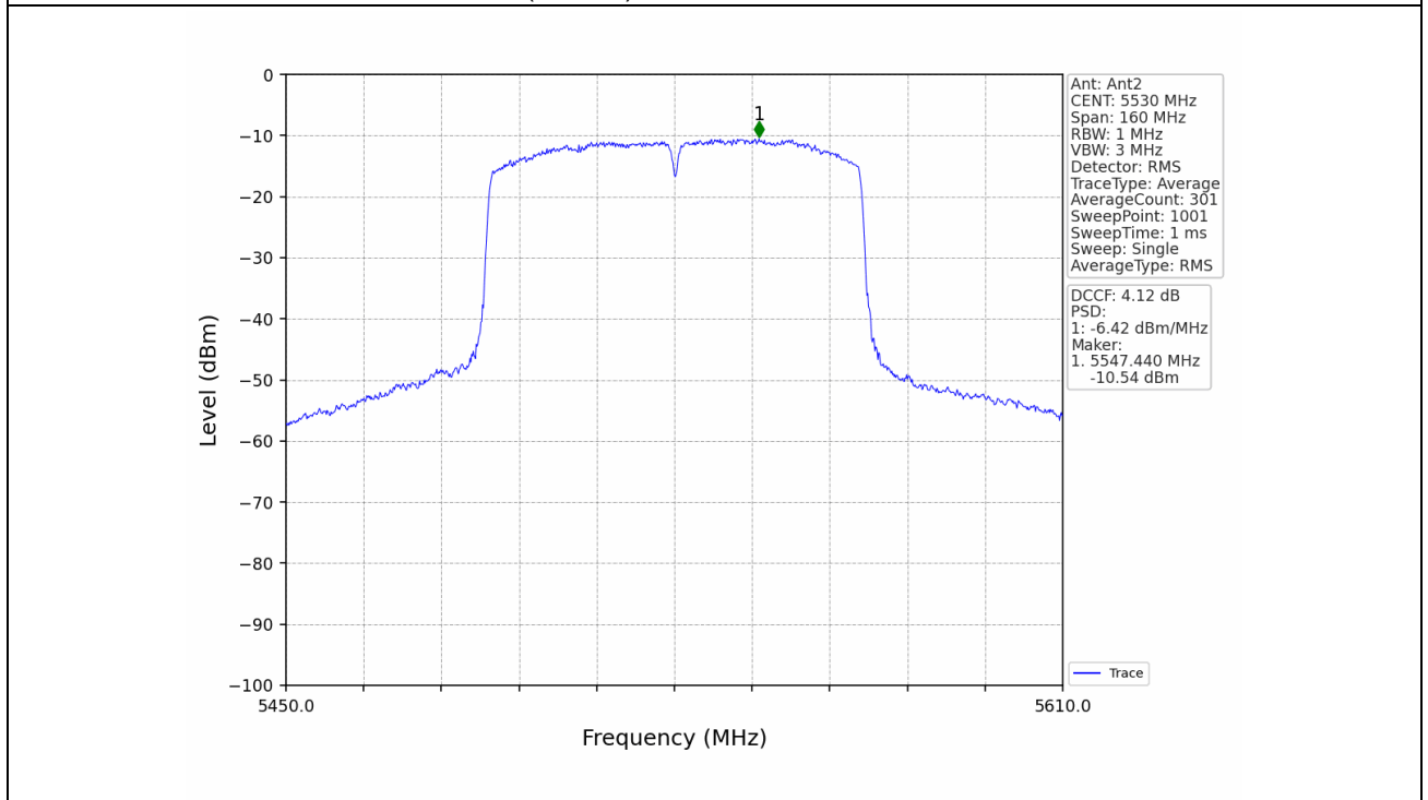
802.11ac(VHT80)_LCH_5530MHz_MIMO_NTNV
