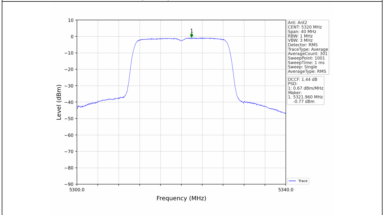
802.11ac(VHT20)_HCH_5320MHz_MIMO_NTNV
