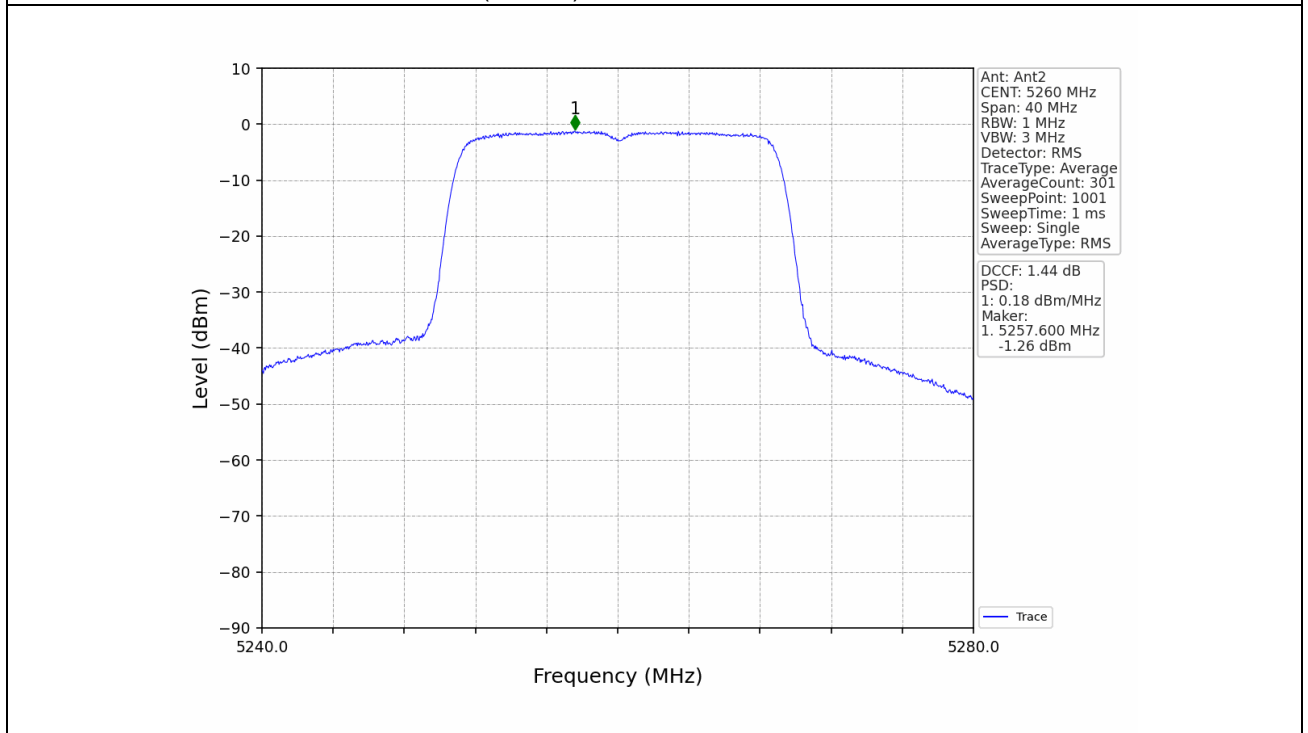
802.11ac(VHT20)_LCH_5260MHz_MIMO_NTNV
