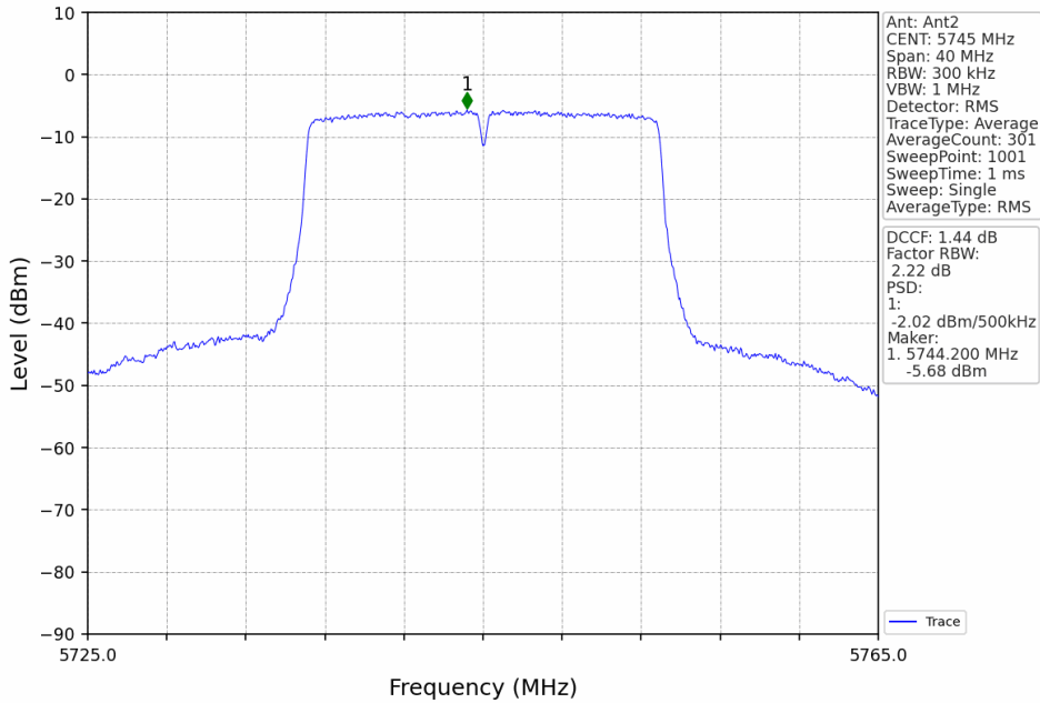
802.11n(HT20)_LCH_5745MHz_MIMO_NTNV
