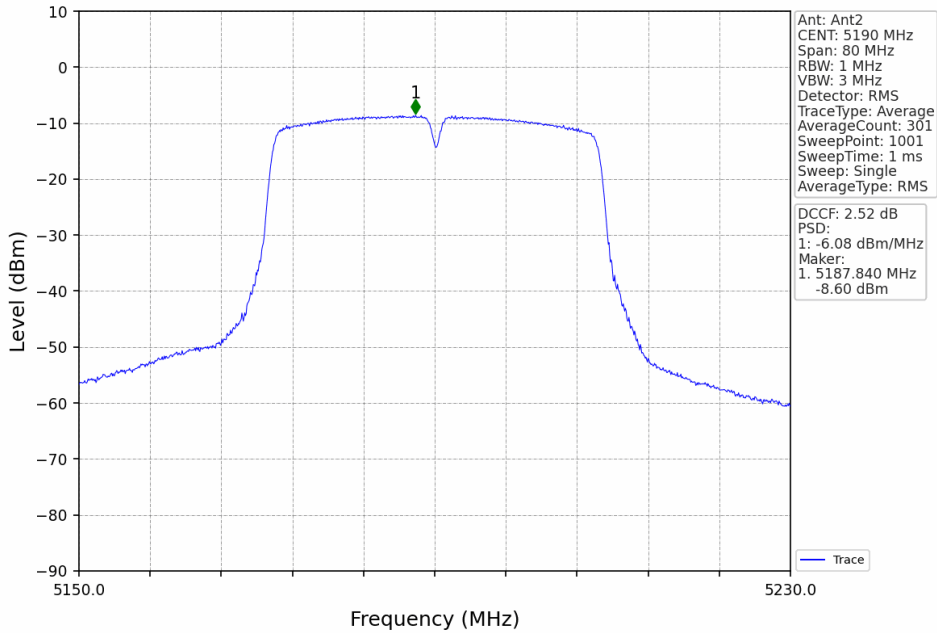
802.11ac(VHT40)_LCH_5190MHz_MIMO_NTNV
