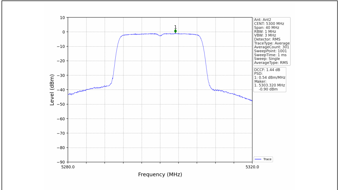
802.11ac(VHT20)_MCH_5300MHz_MIMO_NTNV
