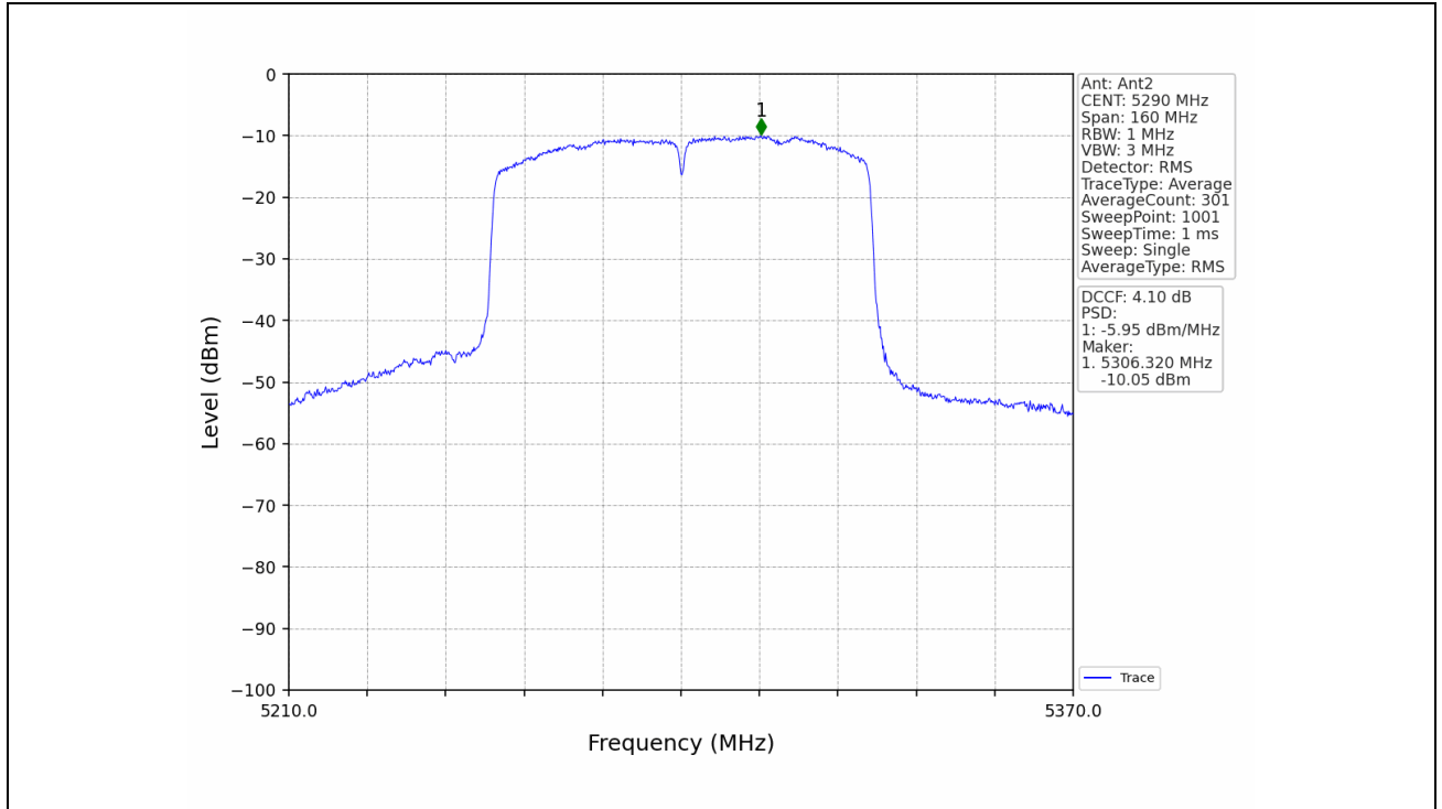
802.11ac(VHT80)_MCH_5290MHz_MIMO_NTNV
