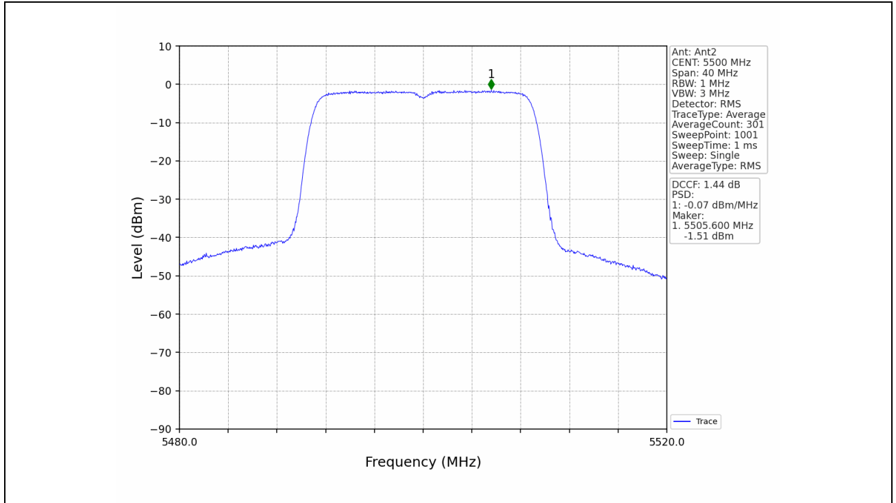
802.11ac(VHT20)_LCH_5500MHz_MIMO_NTNV
