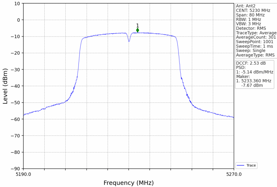
802.11n(HT40)_HCH_5230MHz_MIMO_NTNV
