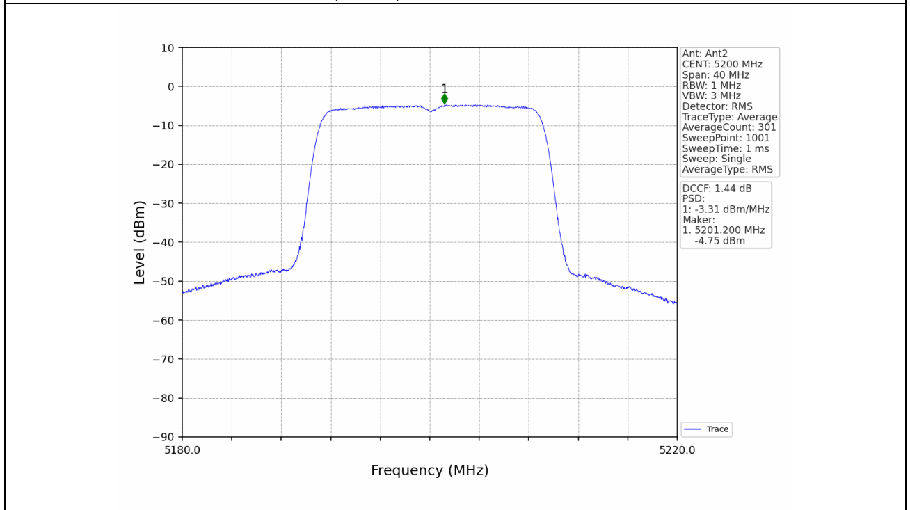
802.11ac(VHT20)_MCH_5200MHz_MIMO_NTNV
