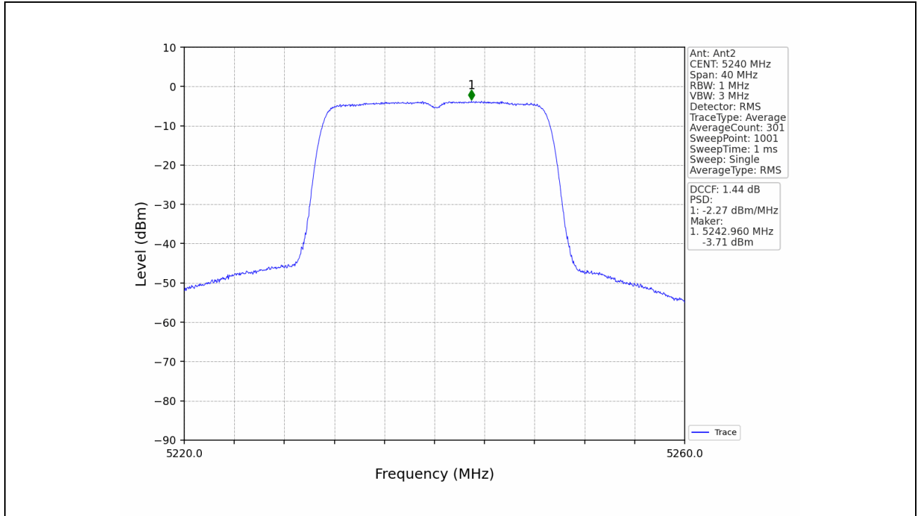
802.11ac(VHT20)_HCH_5240MHz_MIMO_NTNV
