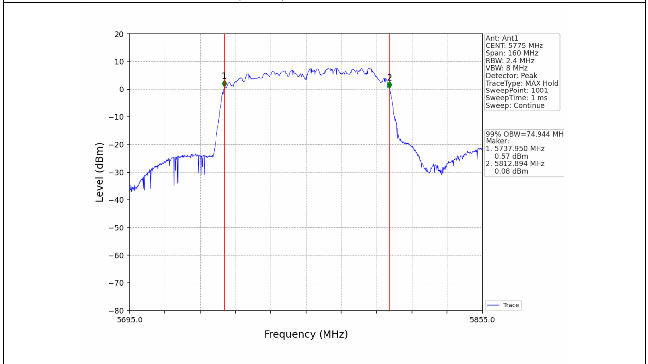
802.11ac(VHT80)_MCH_5775MHz_Ant1_NTNV
