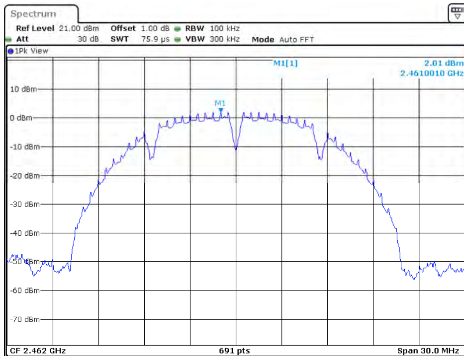
Channel 11 (2462MHz) Reference Level: 2.01dBm
