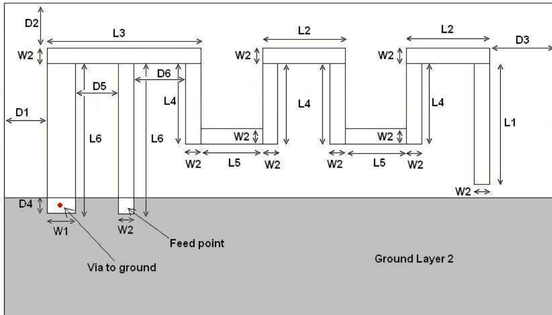
Figure 3: Antenna Dimensions Antenna Gain: 1 dBi
