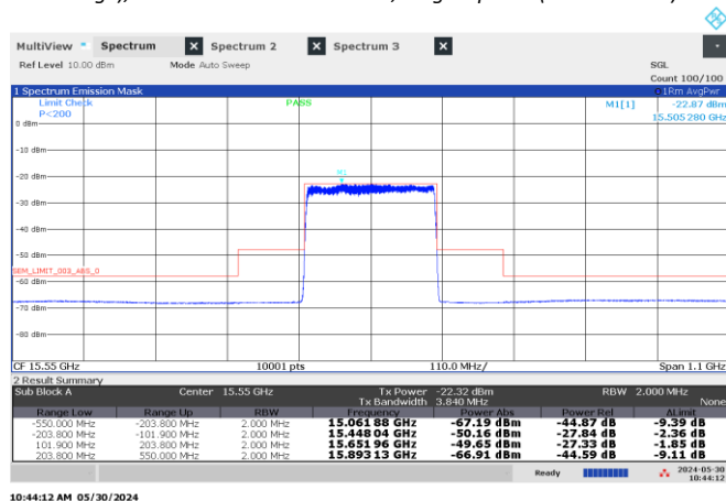
Figure 8.4-23: Emission mask, Middle channel: 15.55 GHz, longest pulse. (200 MHz BW)
