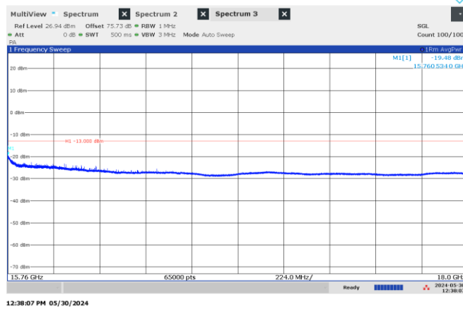
Figure 8.4-33: Emission mask, beyond \pm 250\% of BW (high frequency range), High channel: 15.65 GHz, shortest pulse. (25 MHz BW)
