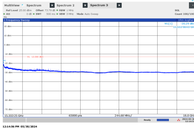
Figure 8.4-27: Emission mask, beyond \pm 250\% of BW (high frequency range), Low channel: 15.45 GHz, shortest pulse. (25 MHz BW)
