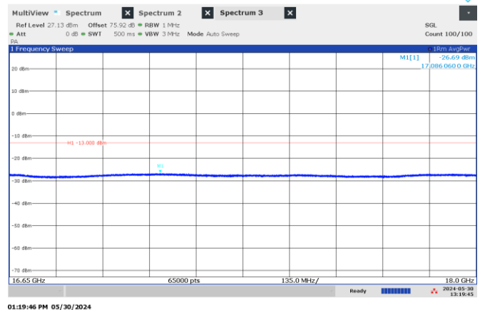
Figure 8.4-36: Emission mask, beyond \pm 250\% of BW (high frequency range), Low channel: 15.50 GHz, shortest pulse. (50 MHz BW)
