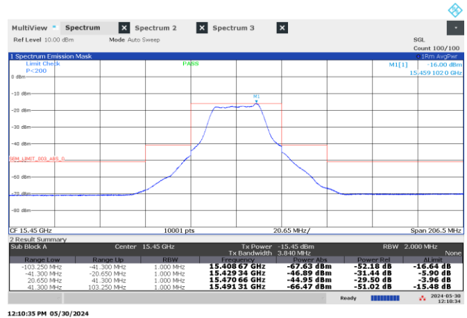
Figure 8.4-26: Emission mask, Low channel: 15.45 GHz, shortest pulse. (25 MHz BW)
