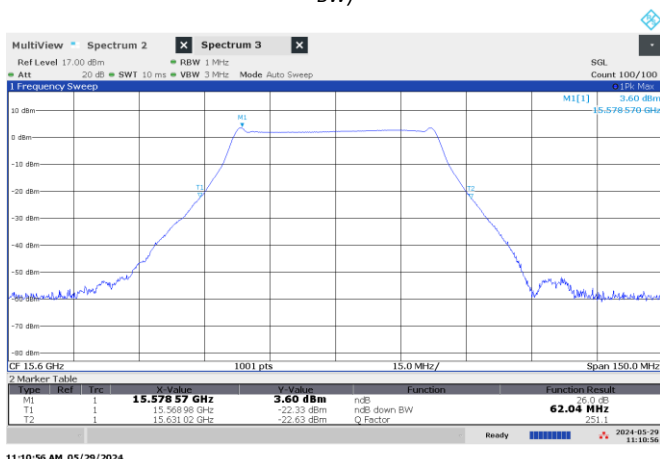
Figure 8.2-14: 26 dB OBW High channel: 15.60 GHz, shortest pulse (50 MHz BW)
