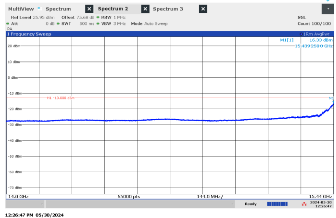
Figure 8.4-28: Emission mask, beyond \pm 250\% of BW (low frequency range), Middle channel: 15.55 GHz, shortest pulse. (25 MHz BW)
