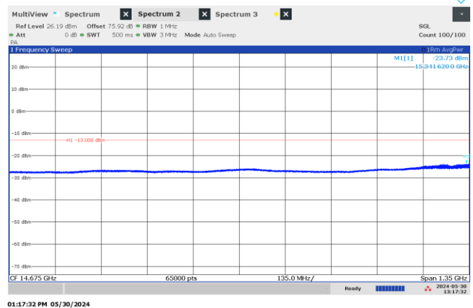
Figure 8.4-34: Emission mask, beyond \pm 250\% of BW (low frequency range), Low channel: 15.50 GHz, shortest pulse. (50 MHz BW)
