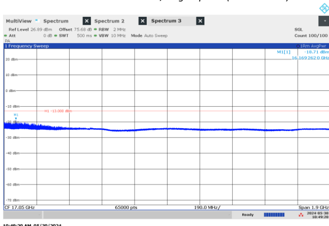
Figure 8.4-24: Emission mask, beyond \pm 250\% of BW (high frequency range), Middle channel: 15.55 GHz, longest pulse. (200 MHz BW)
