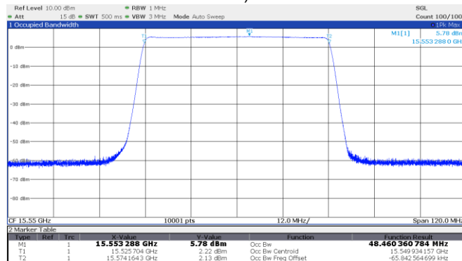
Figure 8.1-5: 99% OBW Middle channel: 15.55 GHz, longest pulse (50 MHz BW)
