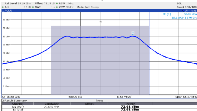
Figure 8.3-11 : EIRP Power, High channel: 15.65 GHz, shortest pulse (25 MHz BW)
