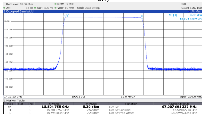
Figure 8.1-7: 99% OBW Middle channel: 15.55 GHz, longest pulse (100 MHz BW)
