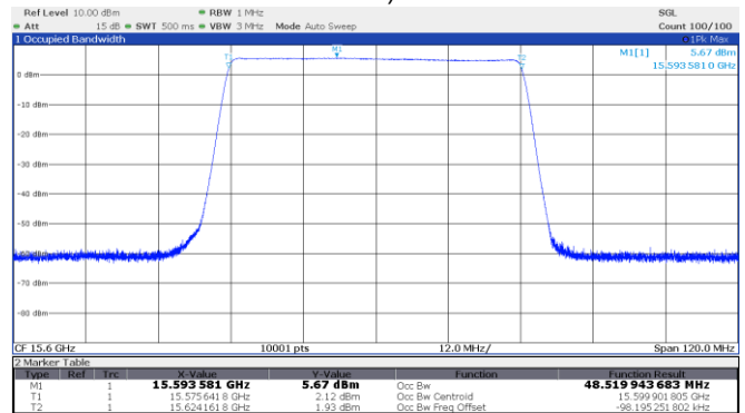
Figure 8.1-6: 99% OBW High channel: 15.60 GHz, longest pulse (50 MHz BW)
