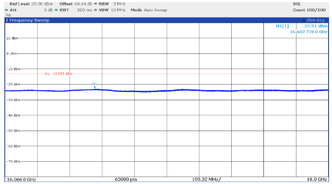
Figure 8.4-48: Emission mask, beyond ±250% of BW (high frequency range), Middle channel: 15.55 GHz, shortest pulse. (200 MHz BW)
