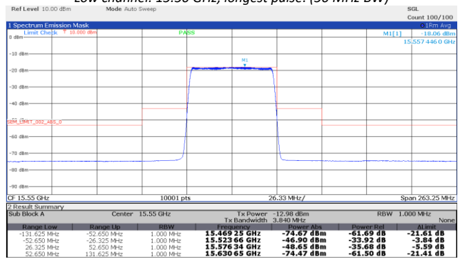
Figure 8.4-14: Emission mask, Middle channel: 15.55 GHz, longest pulse. (50 MHz BW)
