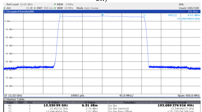
Figure 8.1-8: 99% OBW Middle channel: 15.55 GHz, longest pulse (200 MHz BW)
