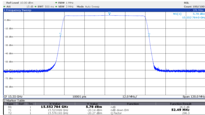
Figure 8.2-5: 26 dB OBW Middle channel: 15.55 GHz, longest pulse (50 MHz BW)
