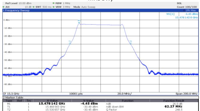
Figure 8.2-12: 26 dB OBW Low channel: 15.50 GHz, shortest pulse (50 MHz BW)
