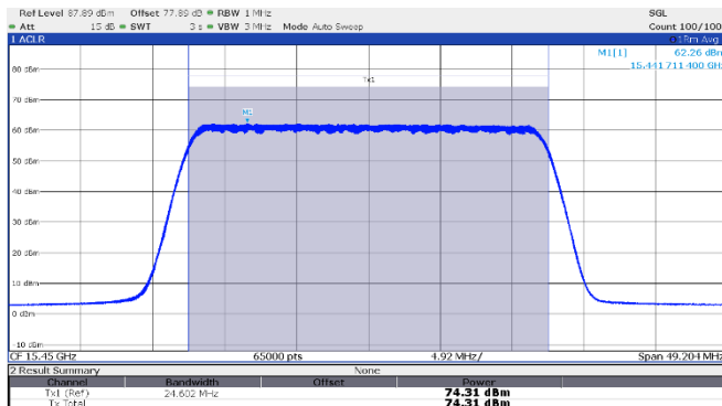
Figure 8.3-1: EIRP Power, Low channel: 15.45 GHz, longest pulse (25 MHz BW)
