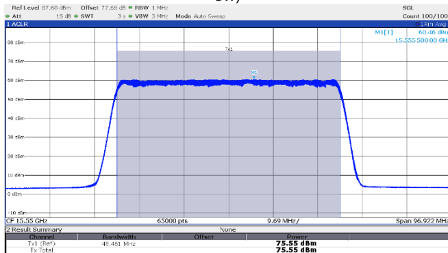
Figure 8.3-5: EIRP Power, Middle channel: 15.55 GHz, longest pulse (50 MHz BW)
