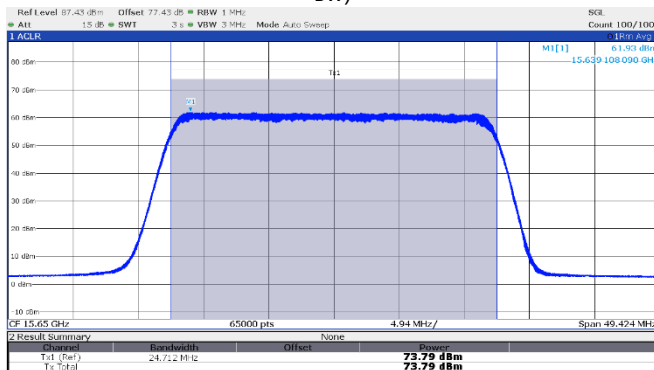
Figure 8.3-3: EIRP Power, High channel: 15.65 GHz, longest pulse (25 MHz BW)
