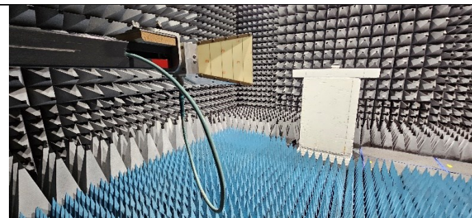
Fig A5: Radiated Emissions
