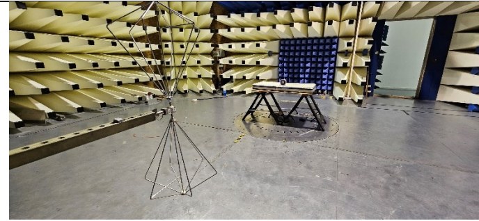
Fig A1: Radiated Emissions
