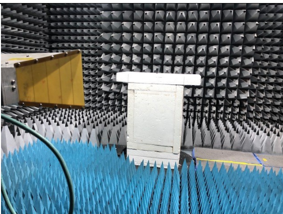
Fig B5: Radiated Emissions 1GHz -18GHz
