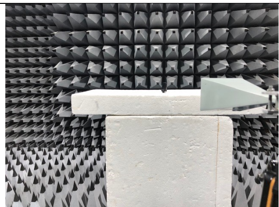
Fig B6: Radiated Emissions > 18GHz
