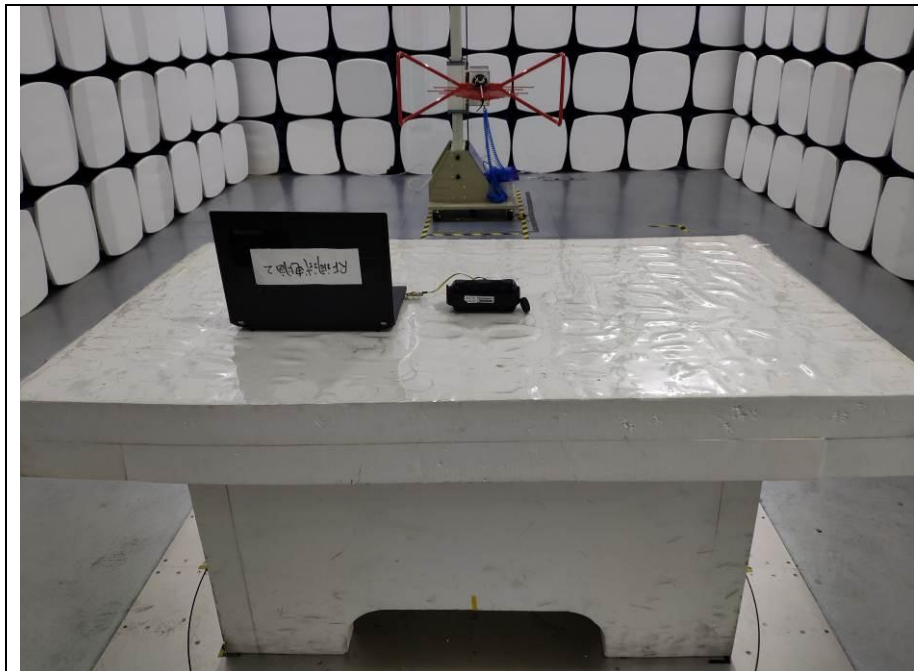
Radiated Emission Frequency Range < 30MHz~1GHz >
