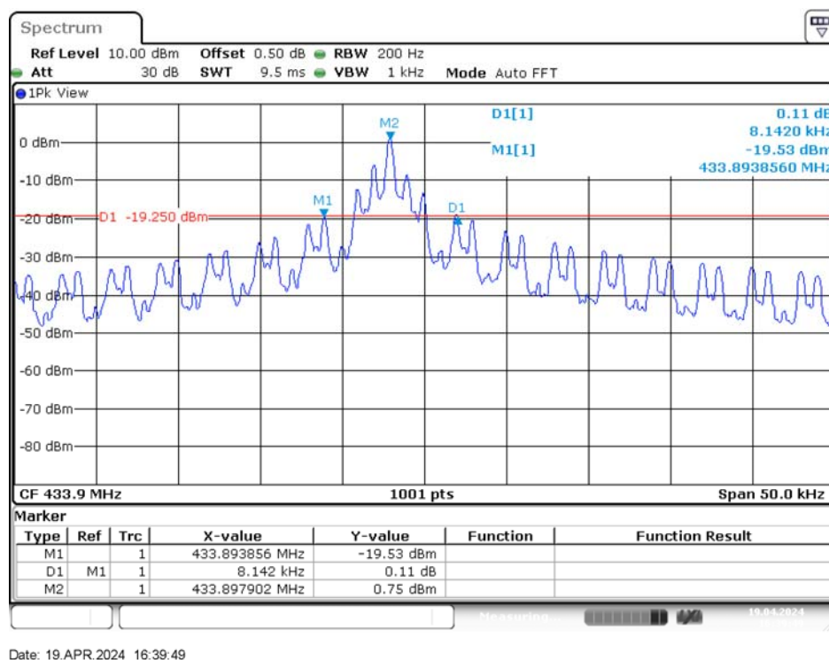
20 dB Emission Bandwidth
