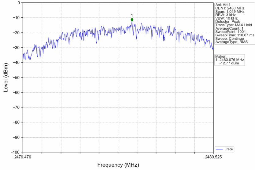
1M_HCH_2480MHz_Ant1_NTNV
