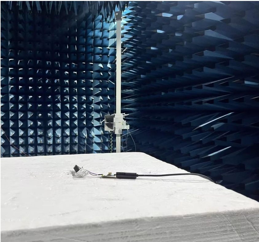
Radiated Spurious Emissions Above 1GHz
