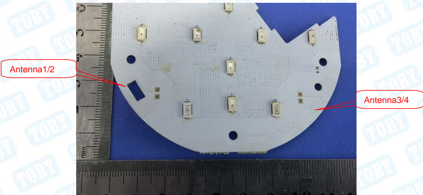
Photo 15 Appearance of PCB
