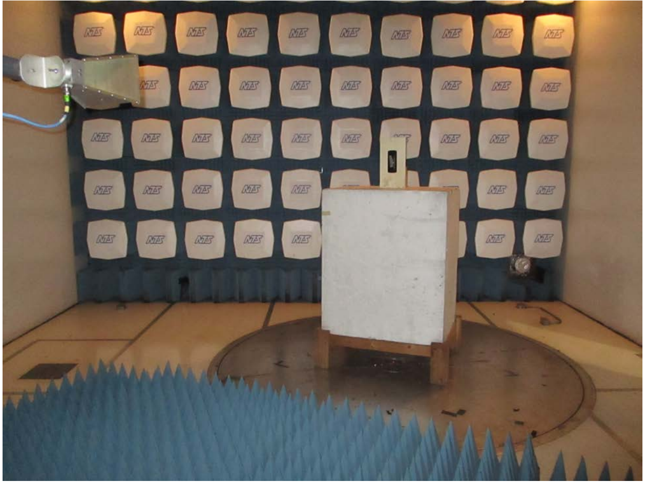
Radiated Measurements Setup 1-10GHz
